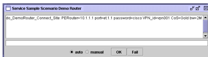
Figure 3-2 DemoRouter GUI
