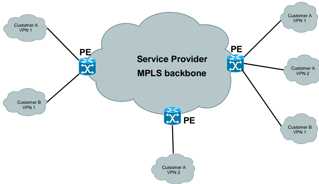
Figure 1-1 Customer site interconnected over an MPLS network
