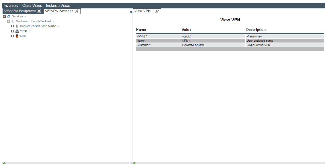
Figure 4-1 Inventory UI
