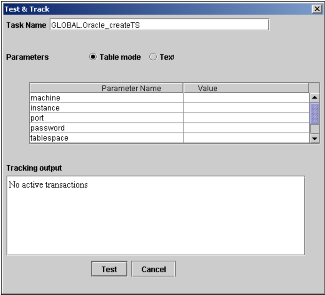
Figure 2-18 Service Builder Test Dialog
