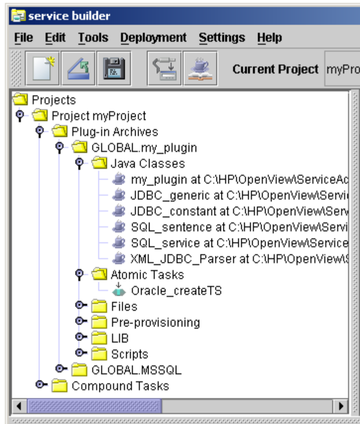
Figure 2–8 Service Builder Project View - After Adding a New Java Class
