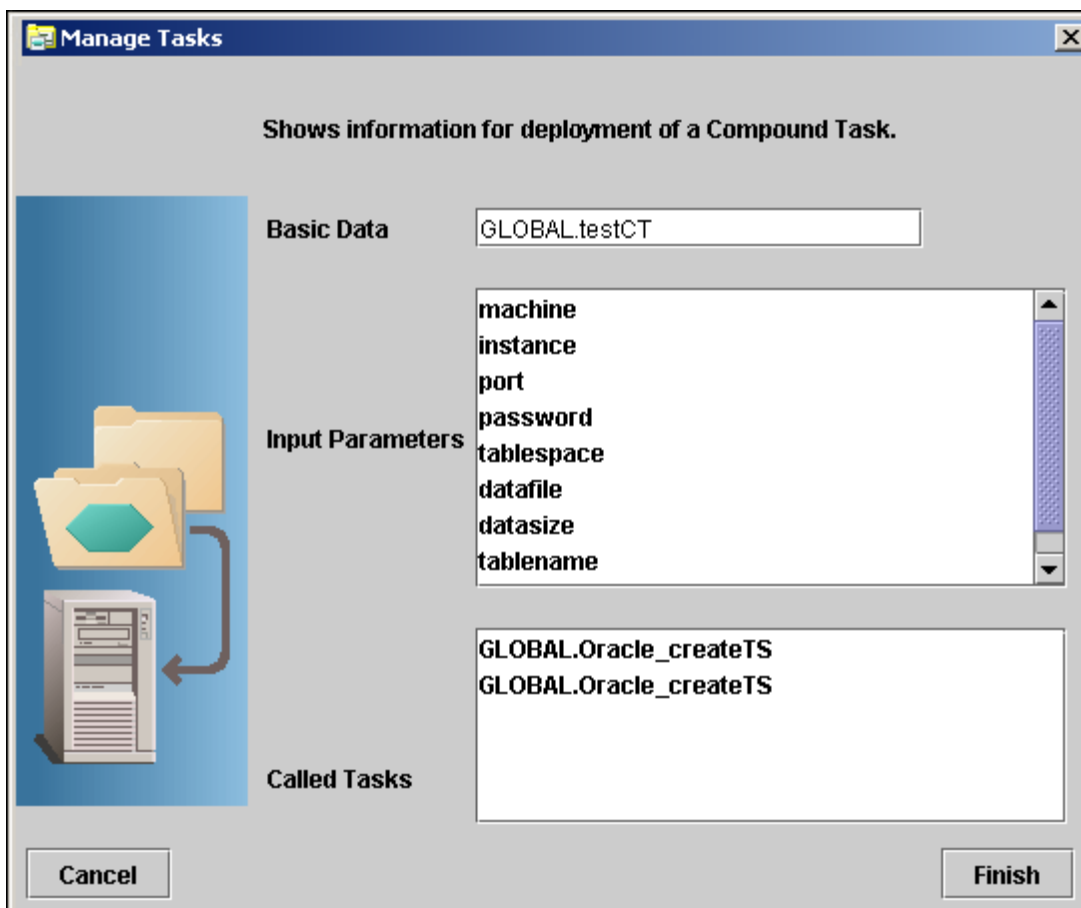
Figure 2–26 Service Builder Compound Task Deployment Dialog
