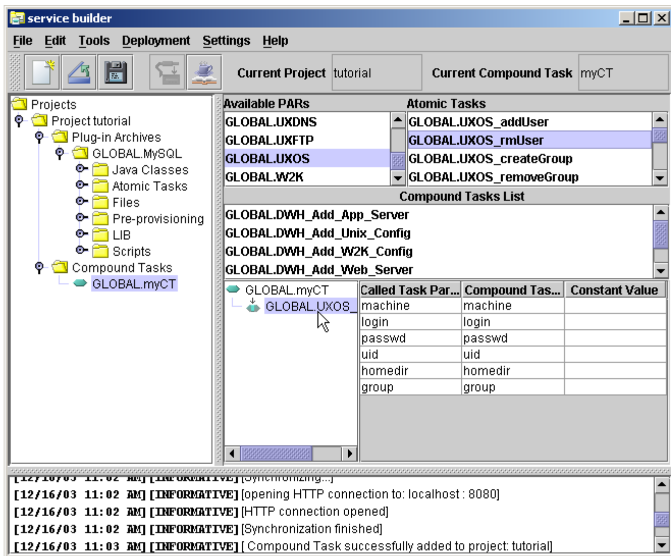
Figure 2-24 Compound Task Work Area with Other Compound Tasks Available
