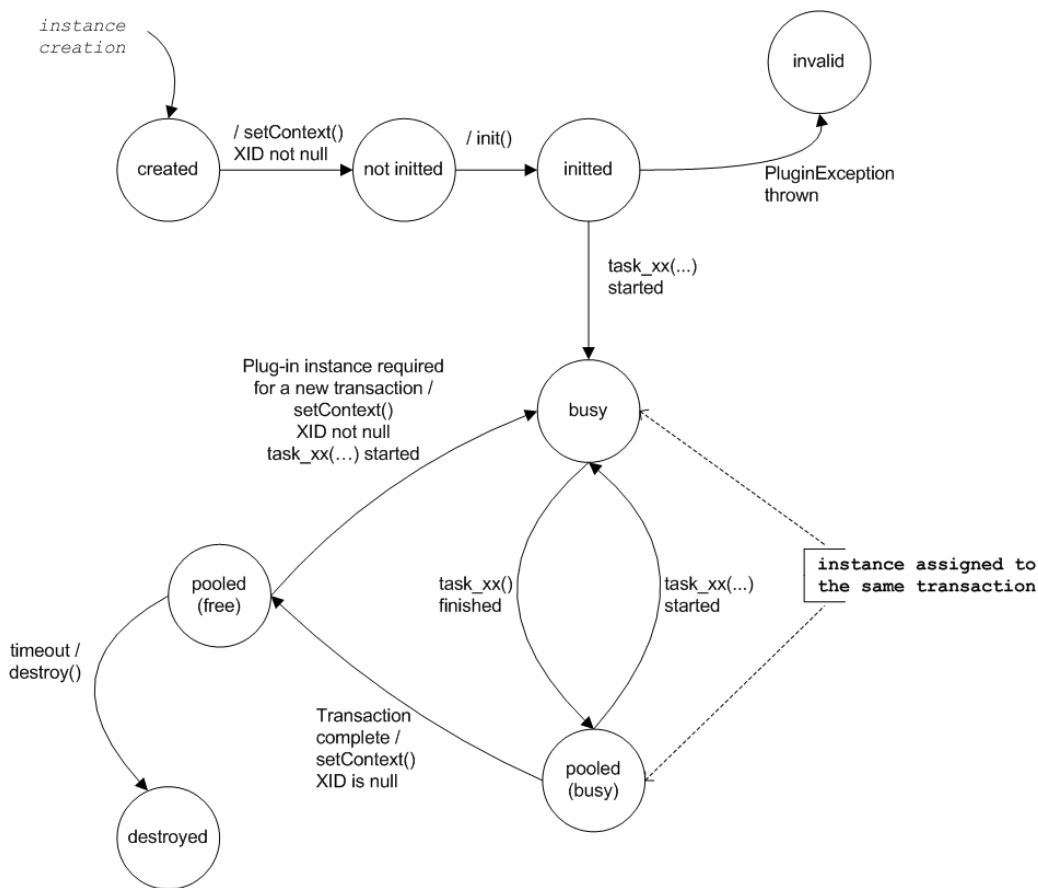
Figure 1-2 Plug-in Life Cycle Diagram
