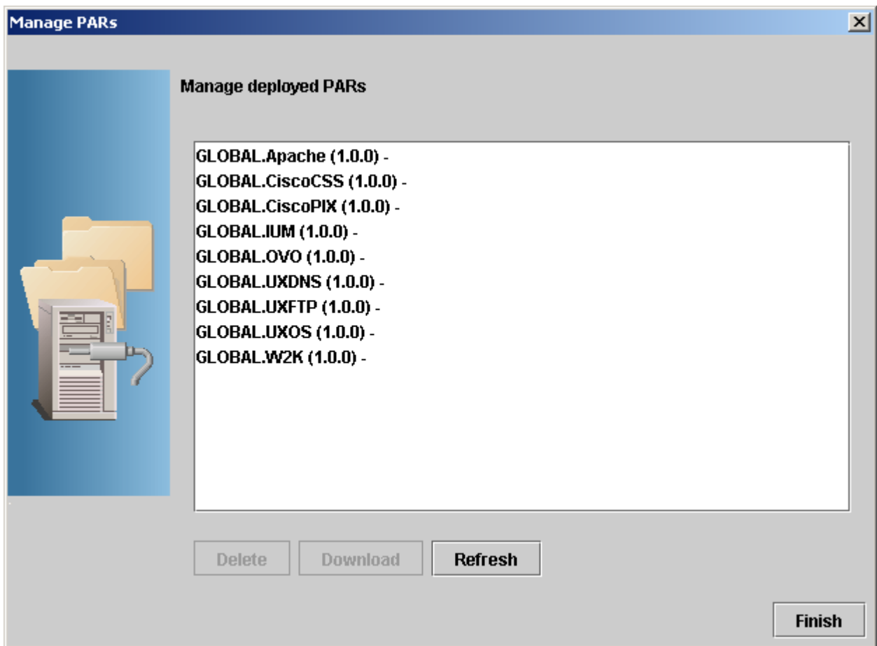
Figure 2-28 Service Builder Manage Plug-in Archives Dialog
