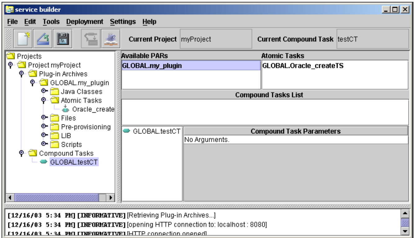
Figure 2–21 Service Builder Compound Task Work Area
