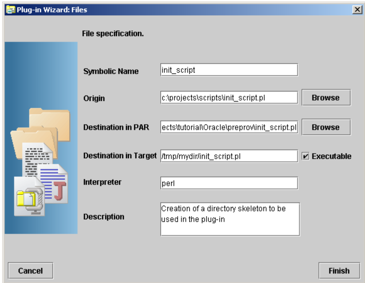
Figure 2-11 Service Builder Files Dialog - Adding Preprovisioning Scripts and Files
