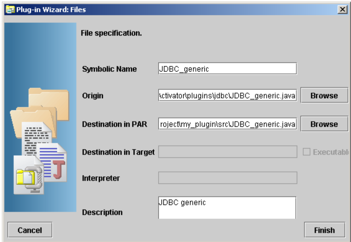
Figure 2-7 Service Builder Files Dialog - Adding a New Java Class
