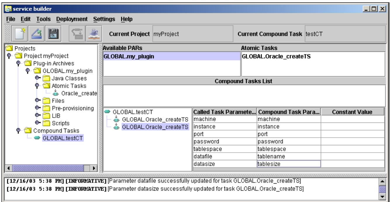
Figure 2-23 Project Directory Structure - After Adding a Compound Task
