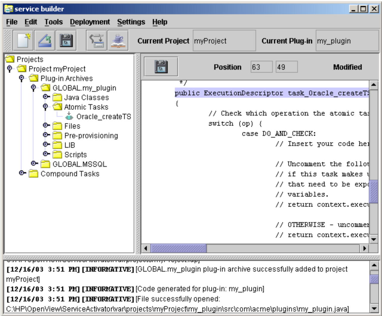
Figure 2-6 Viewing the Java Code for a New Atomic Task
