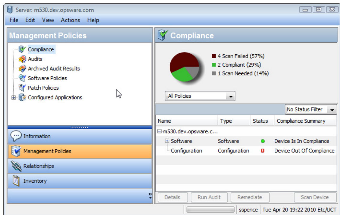
figure 14 Application Configuration Compliance For a Server
