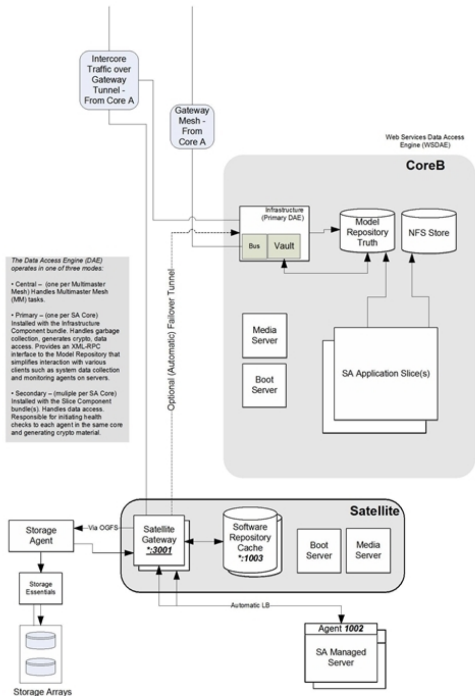
Figure 34. Secondary Core and Satellite
