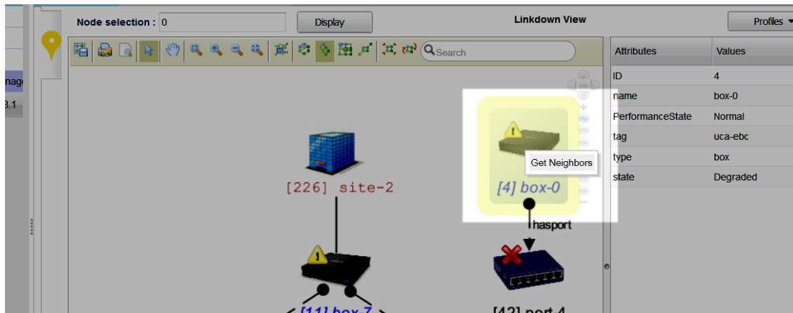
Figure 12 - Get Neighbors action
