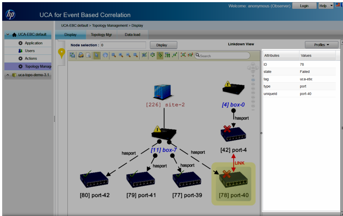
Figure 14 - Inspector view
