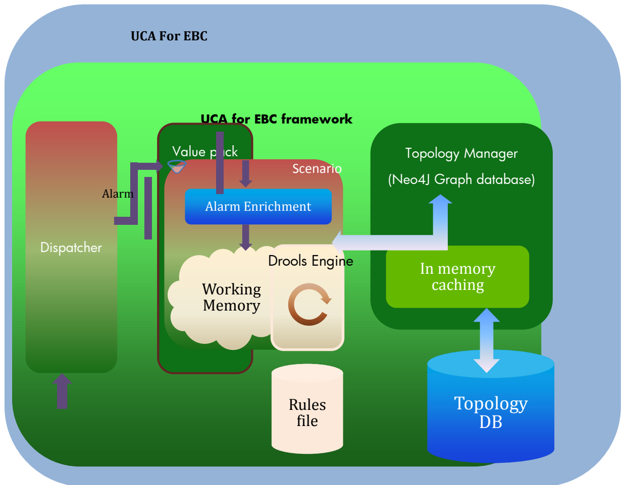
Figure 4 - Alarm enrichment with topology information
