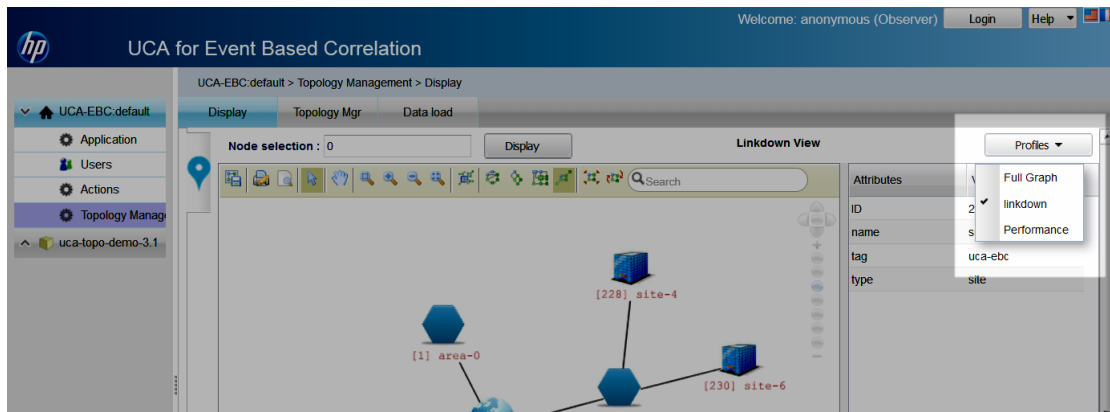
Figure 7 - Profile selection
