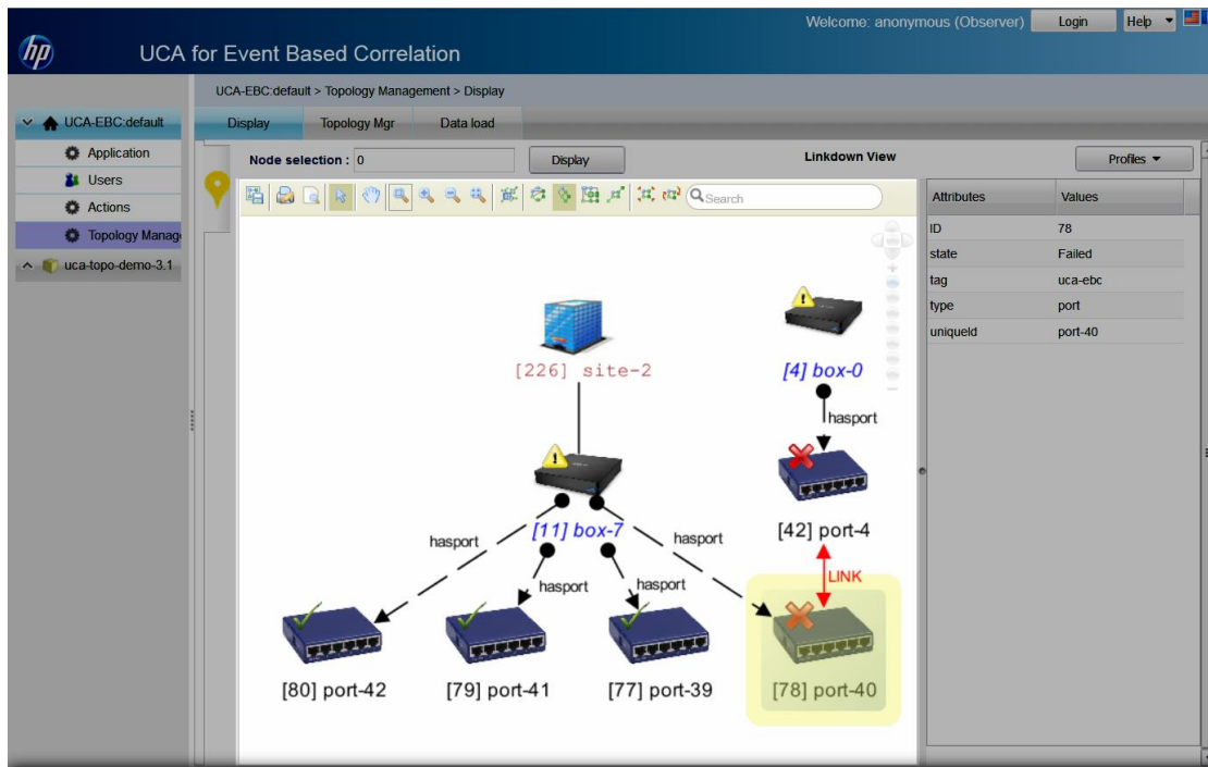
Figure 11 - Drawing the graph from POI
