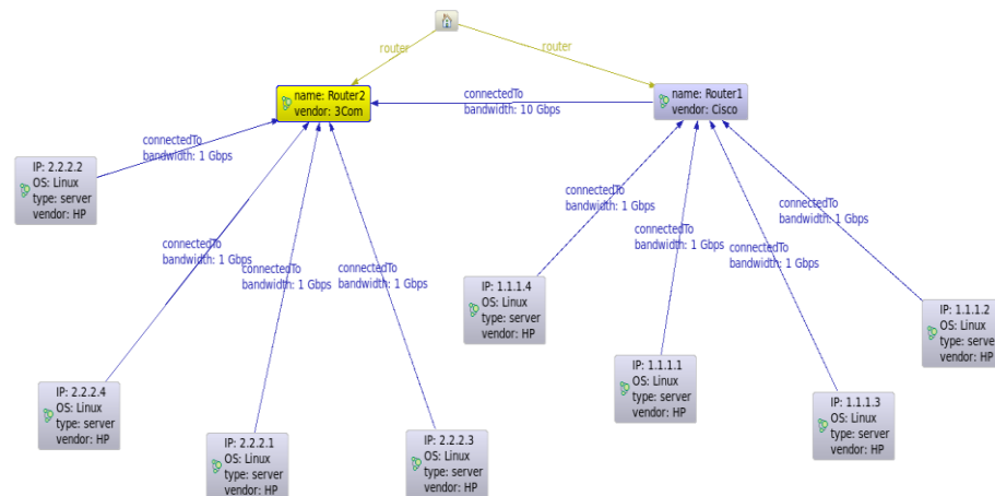
Figure 6 - Graph visualization in Neoclipse
