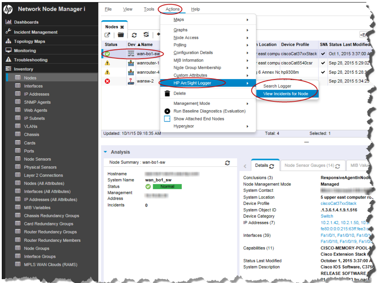
Figure 9 Opening HP ArcSight Logger from a Node or Interface in the Inventory Workspace
