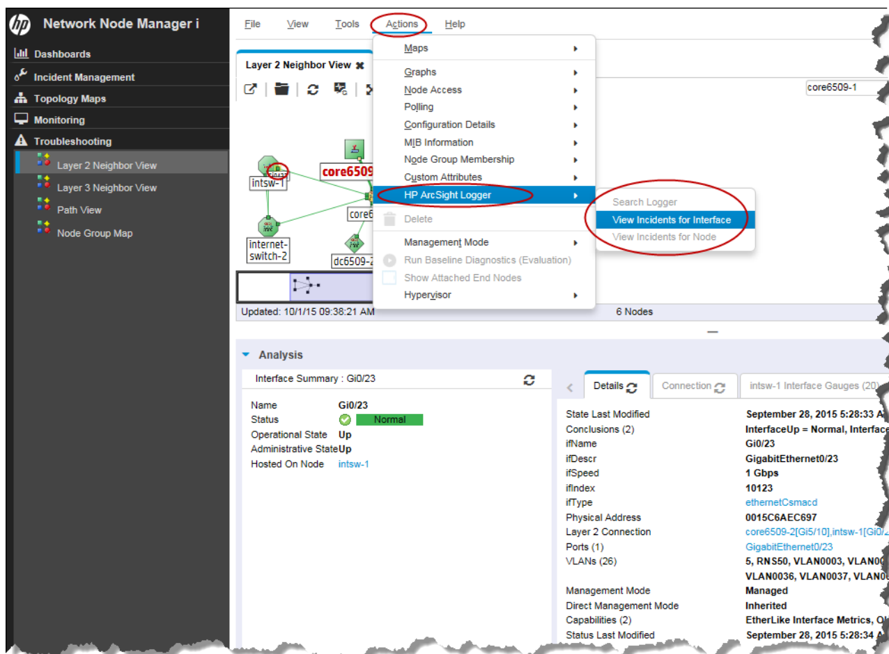
Figure 8 Opening HP ArcSight Logger from an Interface in the Troubleshooting Workspace
