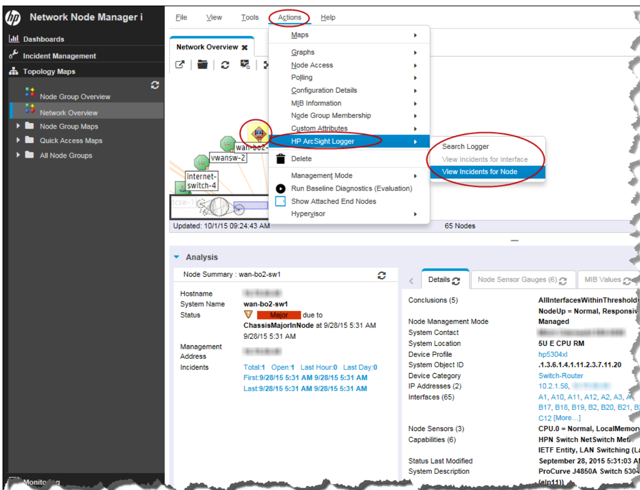
Figure 6 Opening HP ArcSight Logger from a Node in the Topology Maps Workspace
