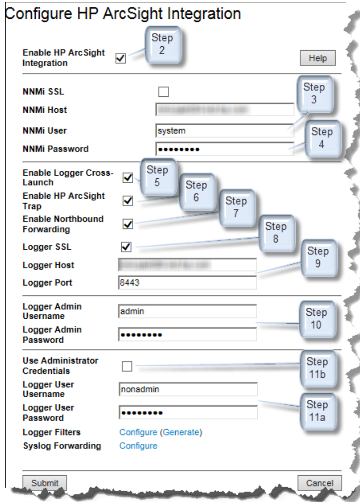
Figure 1 Enabling the HP NNMi-HP ArcSight Logger Integration
