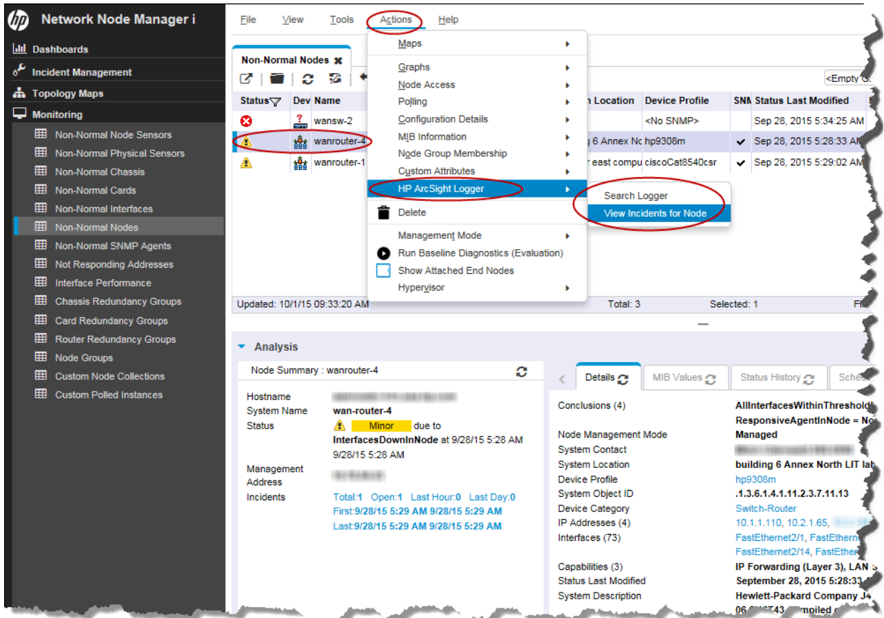
Figure 7 Opening HP ArcSight Logger from a Node in the Monitoring Workspace
