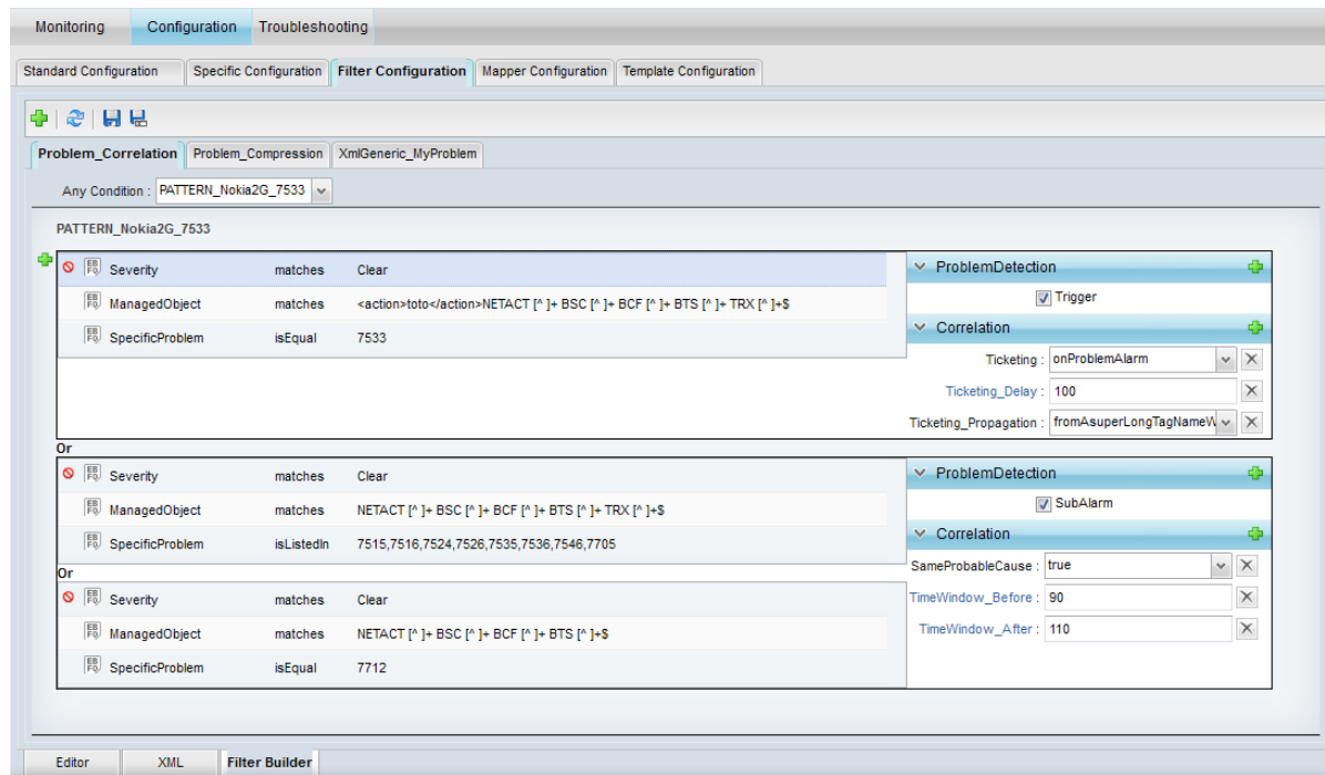
Figure 18 - Scenario Filter Builder Tool
