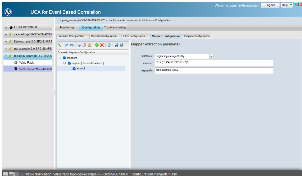
Figure 19 - Scenario mapper configuration
