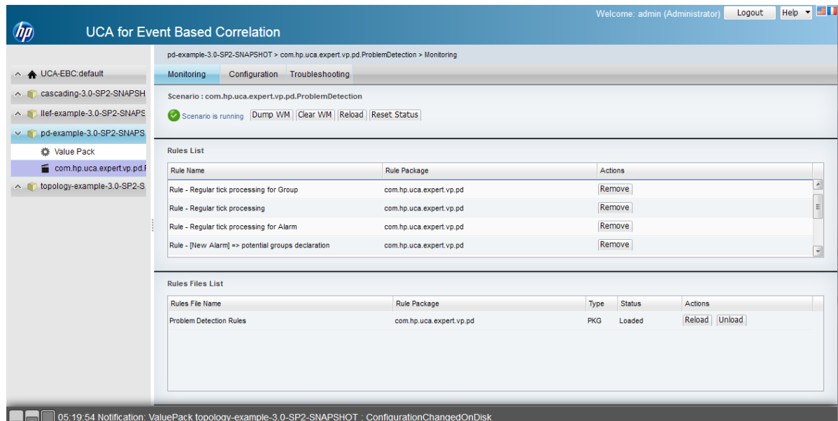
Figure 23 - UCA for EBC Scenario Monitoring View
