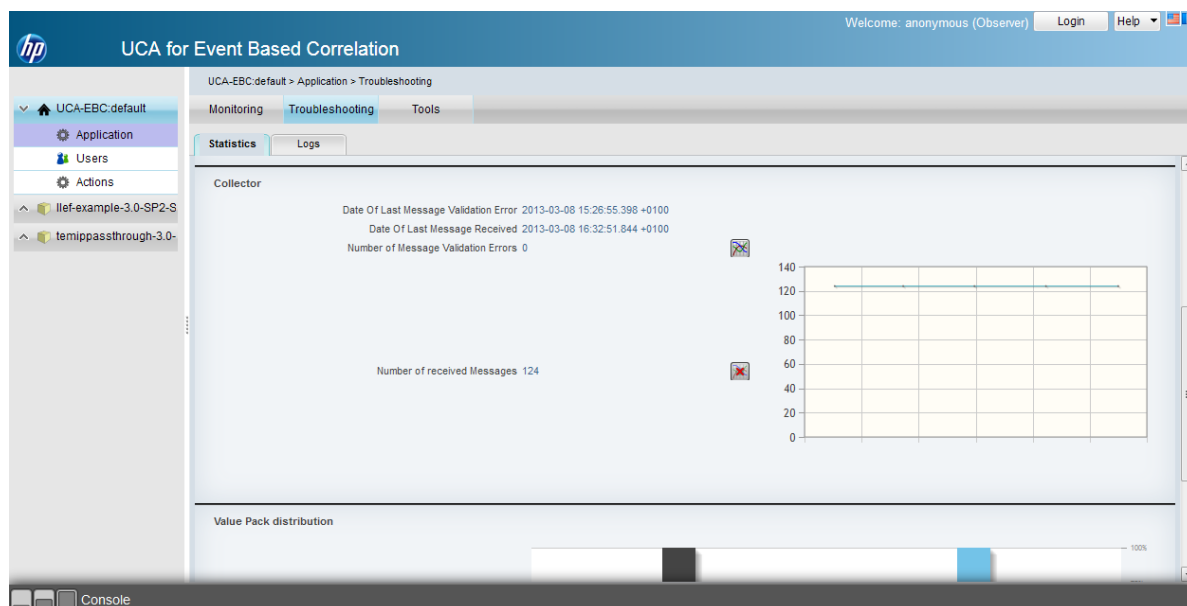
Figure 24 - Statistics content area at Application Level
