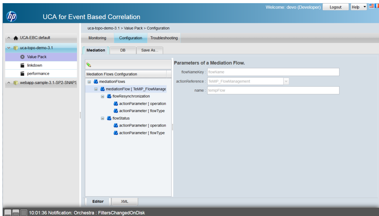
Figure 12 Value Pack Mediation Flows configuration
