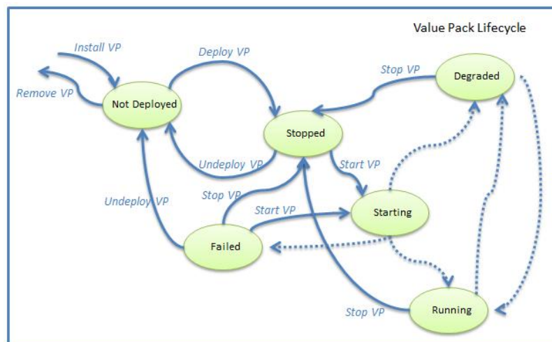
Figure 8 - Value Pack life cycle
