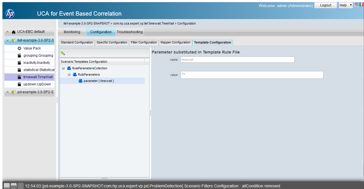
Figure 20 - Scenario template configuration
