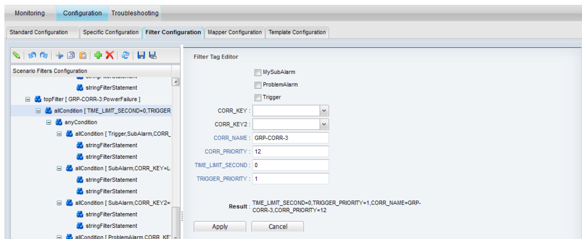
Figure 17 - Scenario Filter Tag Editor
