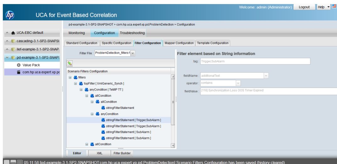
Figure 15 - Scenario Filter Configuration
