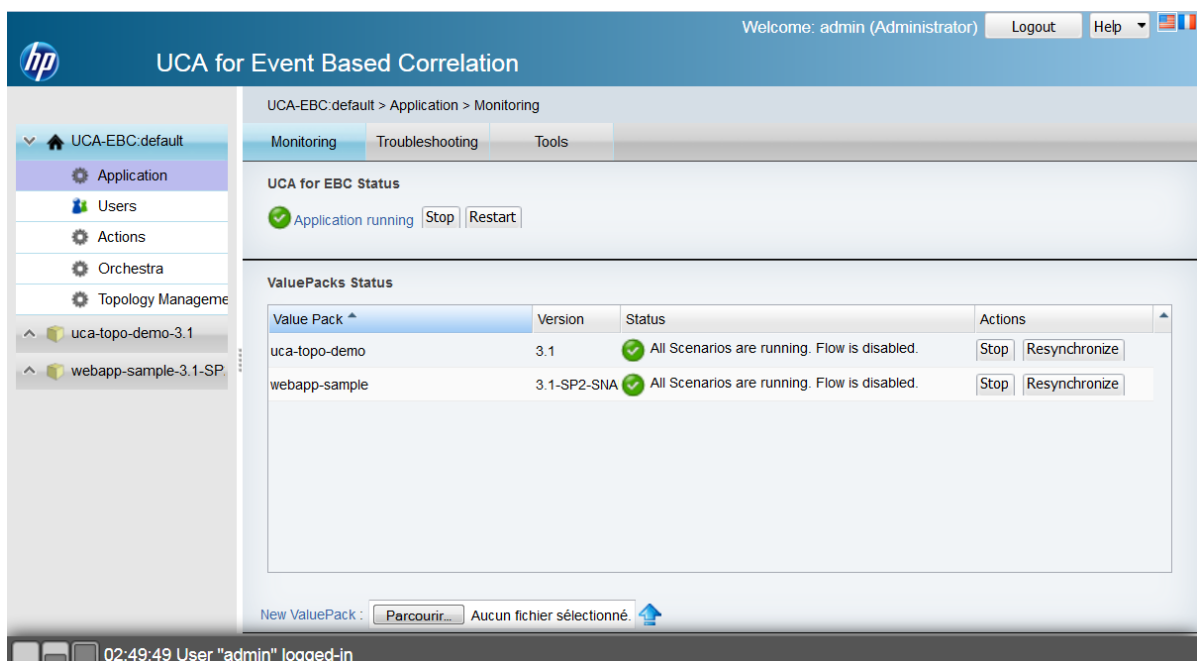
Figure 7 - UCA for EBC Application level operations
