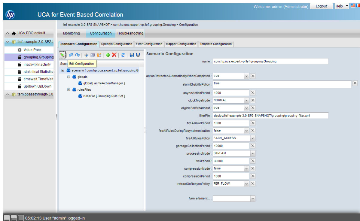
Figure 9 - Standard scenario configuration – Edit mode
