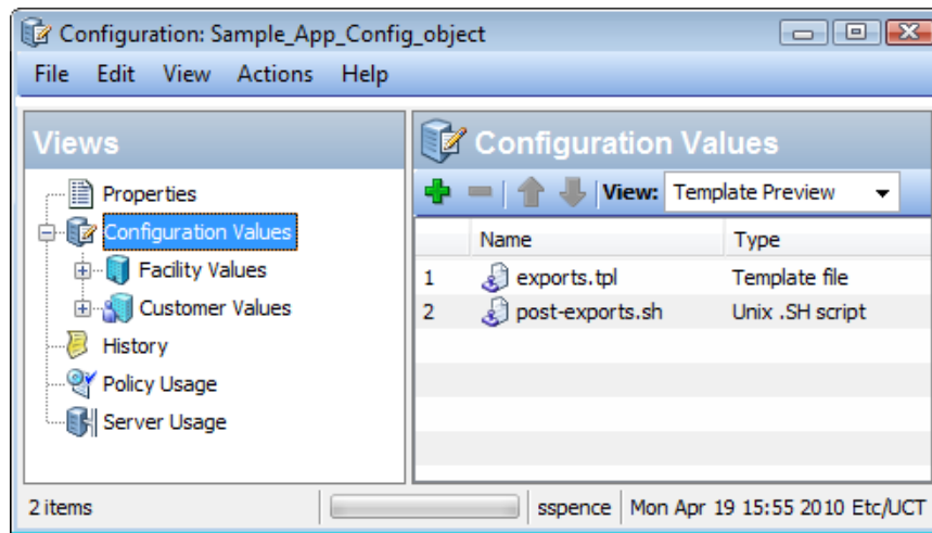
figure 8 Application Configuration Containing a Configuration Template and a Shell Script
