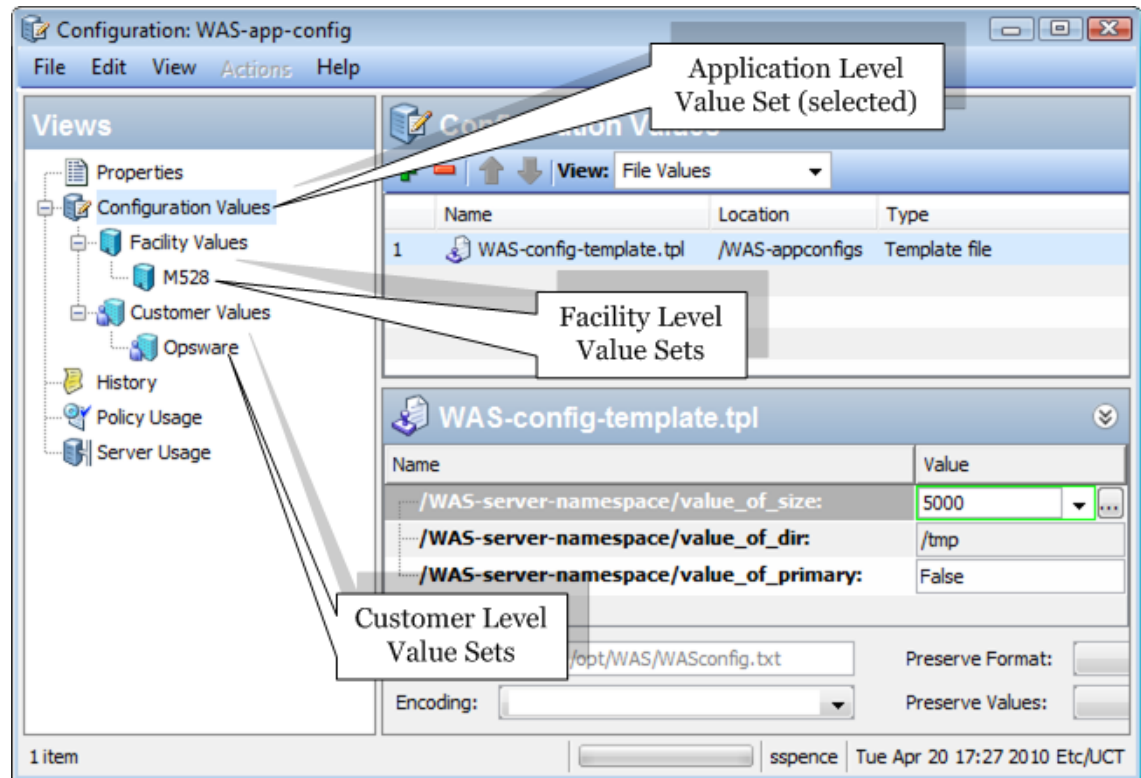
figure 11 Value Set Editor at the Application, Facility and Customer Levels - Application Level Selected
