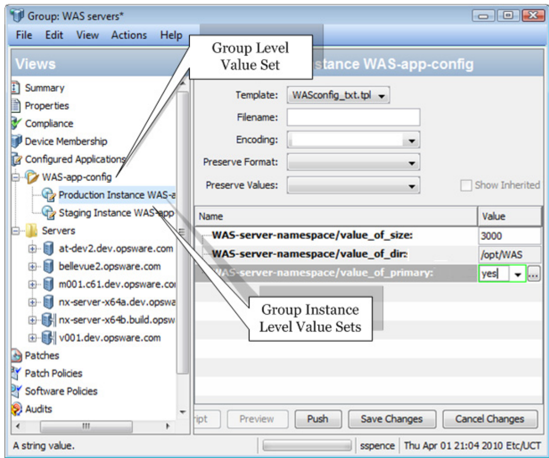
figure 12 Value Set Editor at the Group Level and the Group Instance Level, Displaying Values for the Instance “Production Instance WAS-appconfig”
