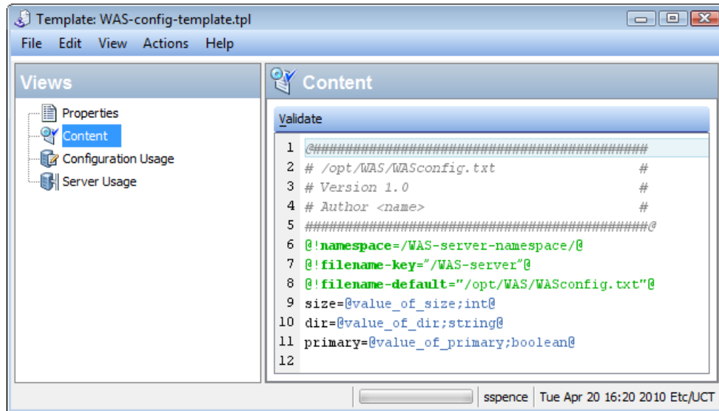
figure 9 Example Configuration Template Written in CML
