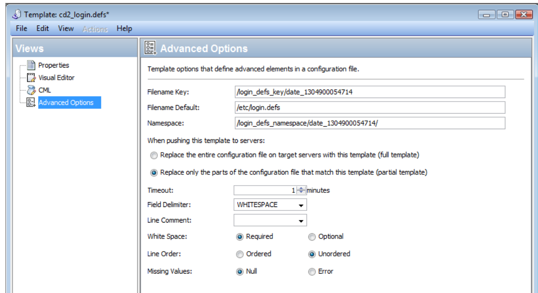
figure 7 Advanced Options in the Visual Editor
