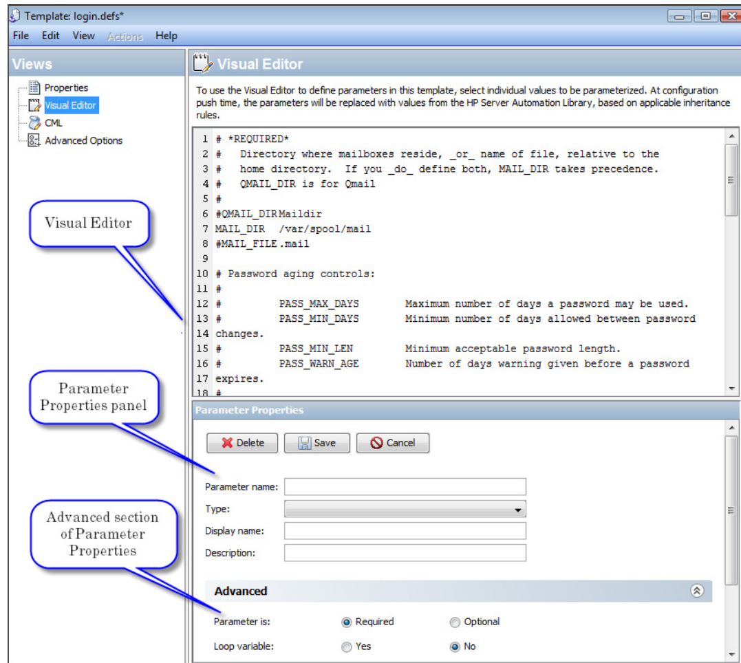
figure 3 Visual Editor Interface
