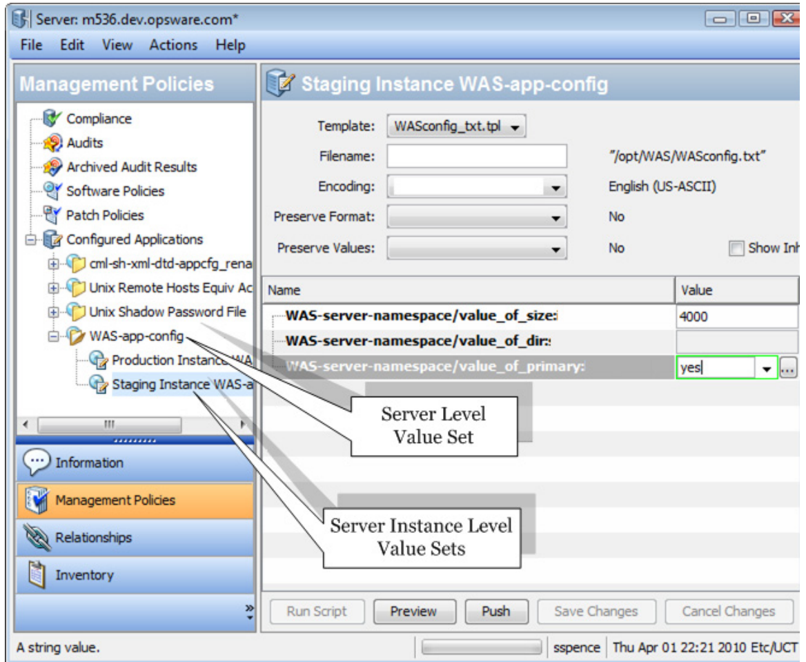
figure 13 Value Set Editor at the Server Level and the Server Instance Level, Displaying Values for the Instance “Staging Instance WAS-appconfig”
