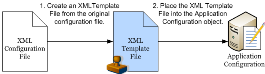
figure 18 XML Configuration Files
