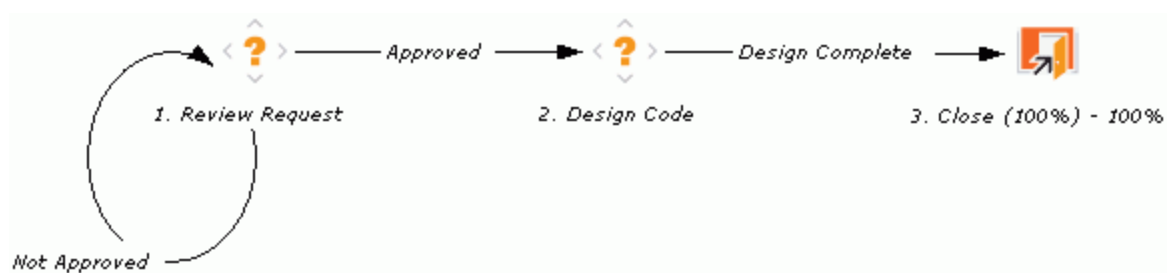
Figure 3-11. Transitioning back to the same step
