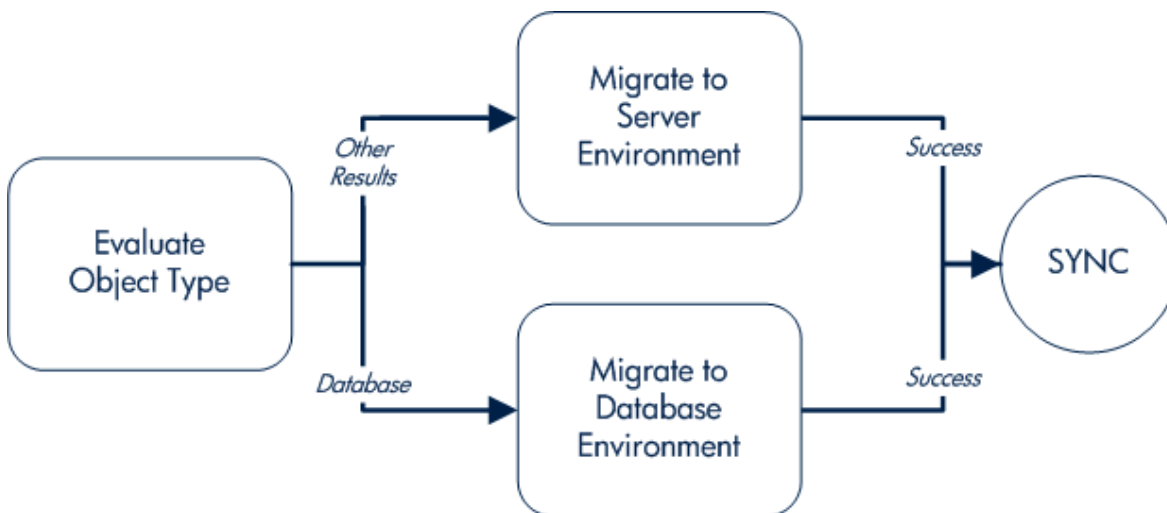
Figure 4-1. Transitioning based on a token
