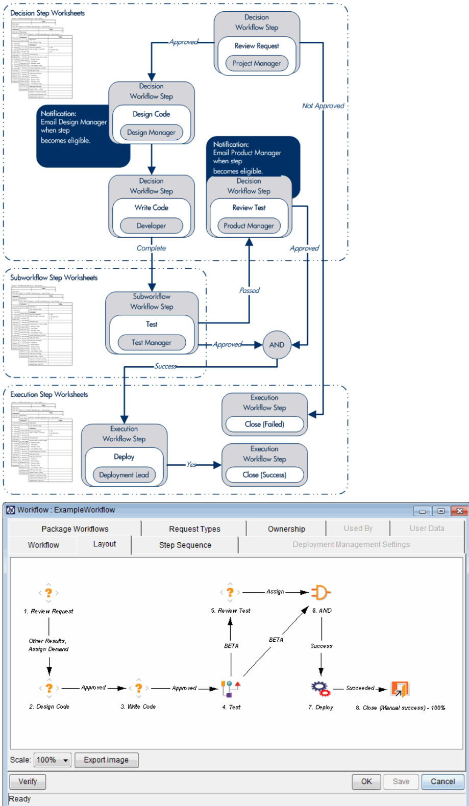
Figure 3-2. Stage 2. Create the workflow
