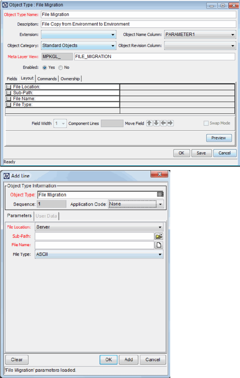
Figure 5-4. Example of an object type and Layout tab
