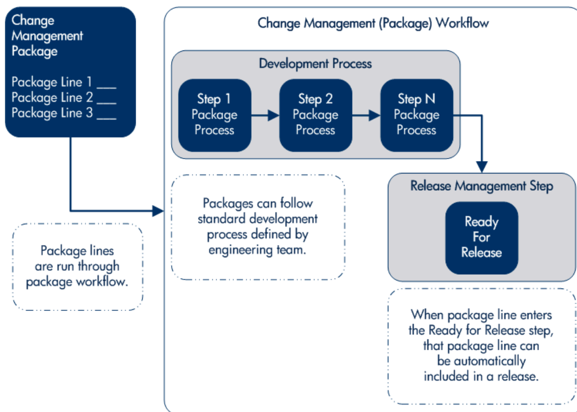
Figure 6-1. Ready for release step in workflow
