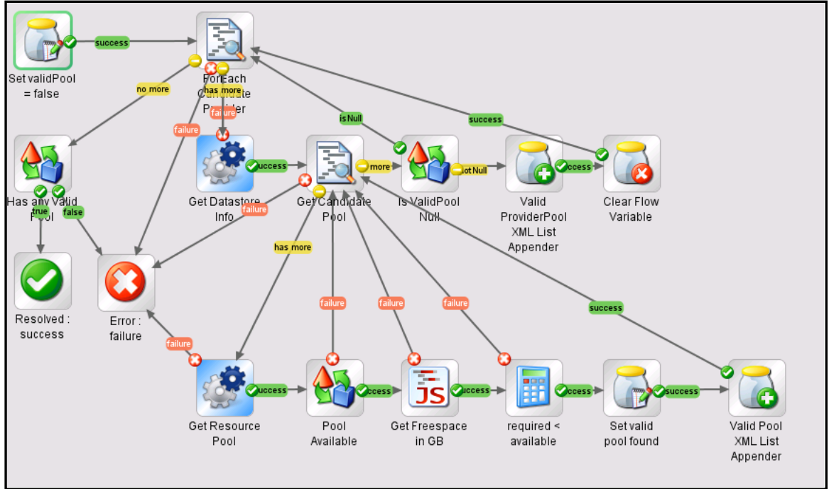
Figure 22. Create Valid Provider and Pool list
