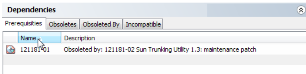
figure 21 Patch Dependencies
