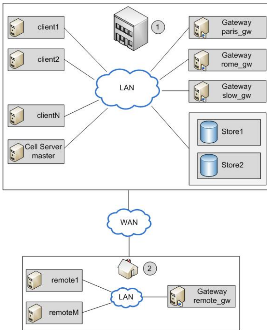
Figure 7: Deployment example within a central office/ remote office environment
