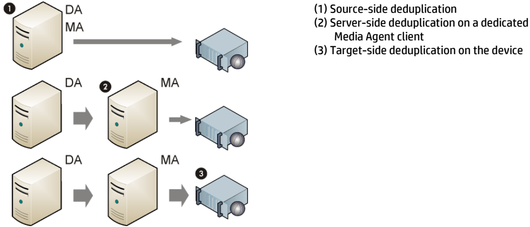
Figure 1: Deduplication setups
