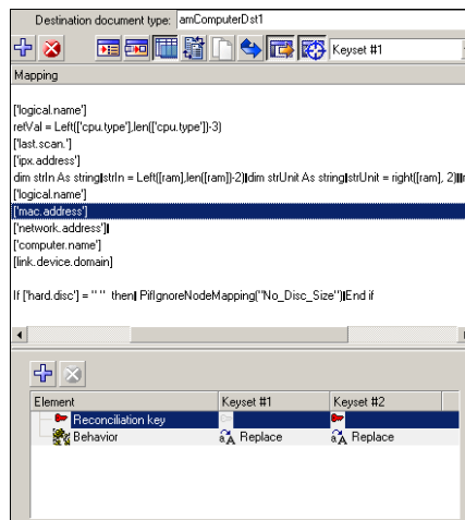
Mac address as the reconciliation key
