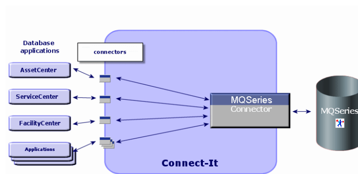
IBM Websphere MQ connector
