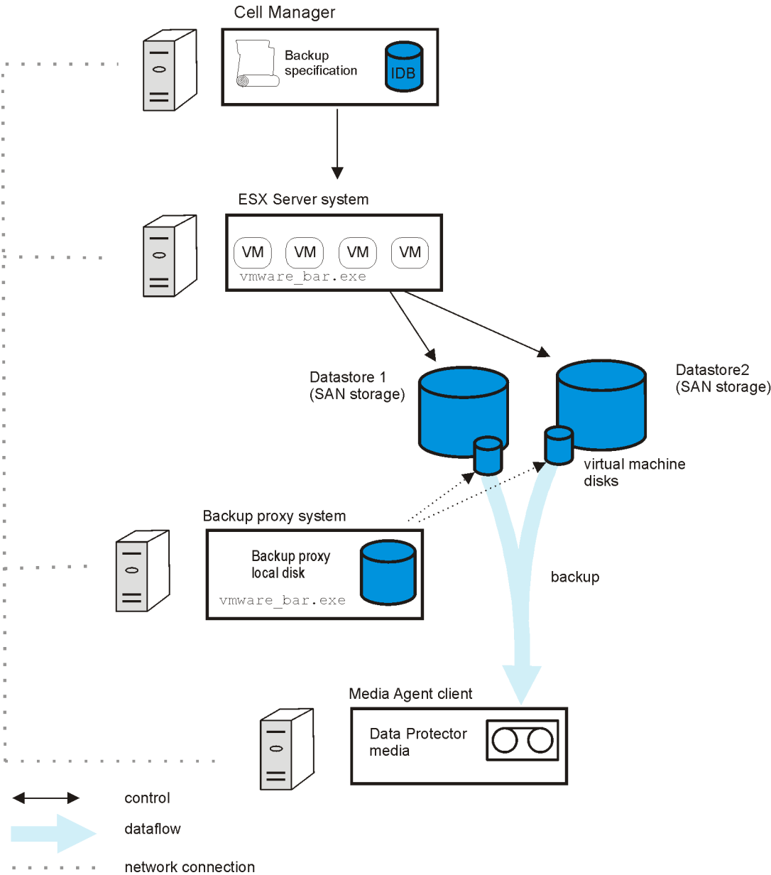
Figure 57 VCBfile method
