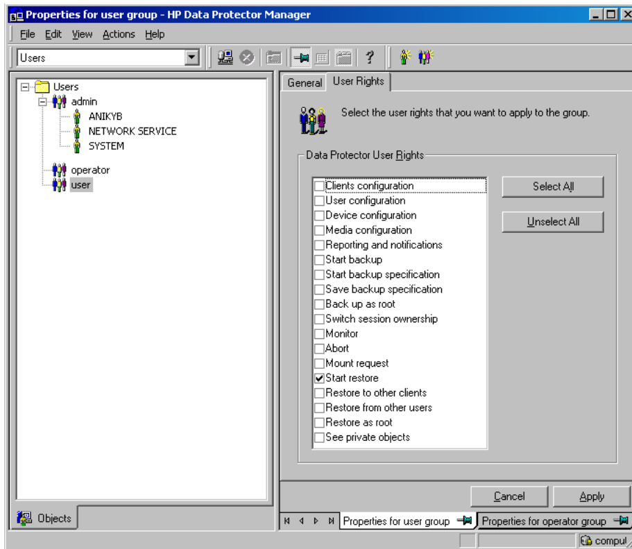
Figure 6 Data Protector user rights
