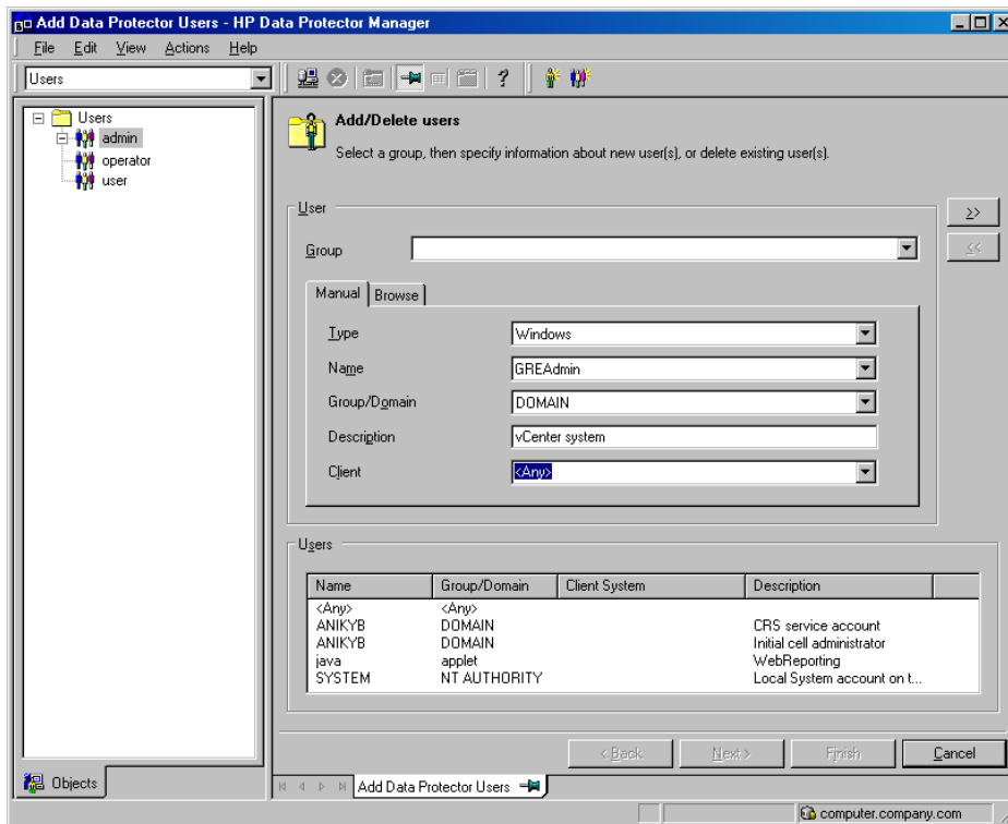
Figure 5 Adding user domain information
