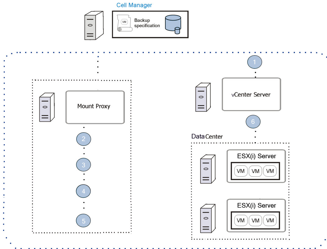
Figure 9 Restore and recovery flow
