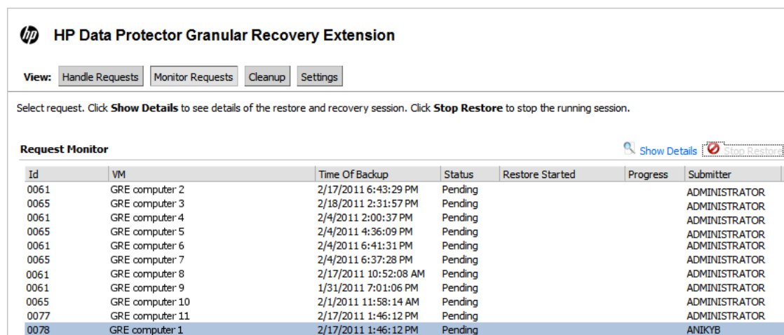
Figure 27 Stopping pending sessions
