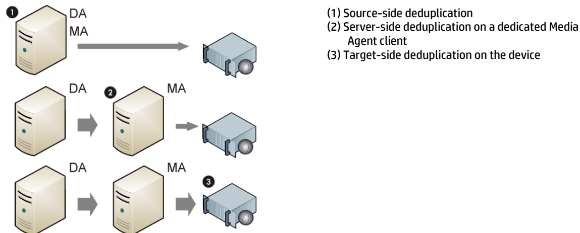
Figure 1: Deduplication setups
