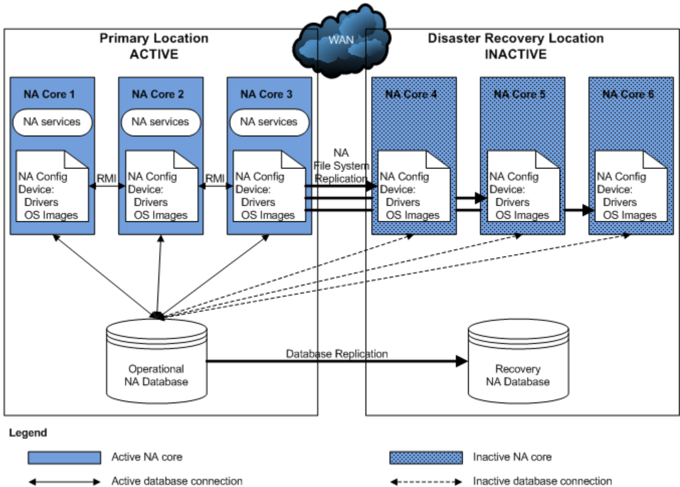
Figure 1 Example NA Disaster Recovery Architecture
