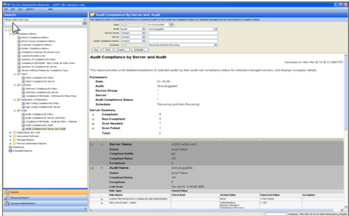
Figure 25 Audit Compliance By Server and Audit - Value-Based Checks
