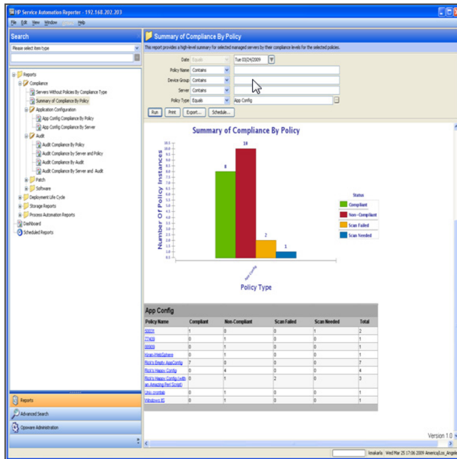
Figure 15 Summary of Compliance By Policy
