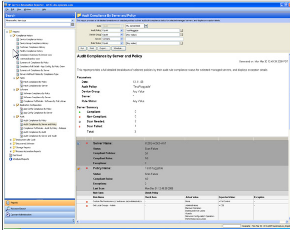
Figure 23 Audit Compliance By Server and Policy - Value-Based Checks
