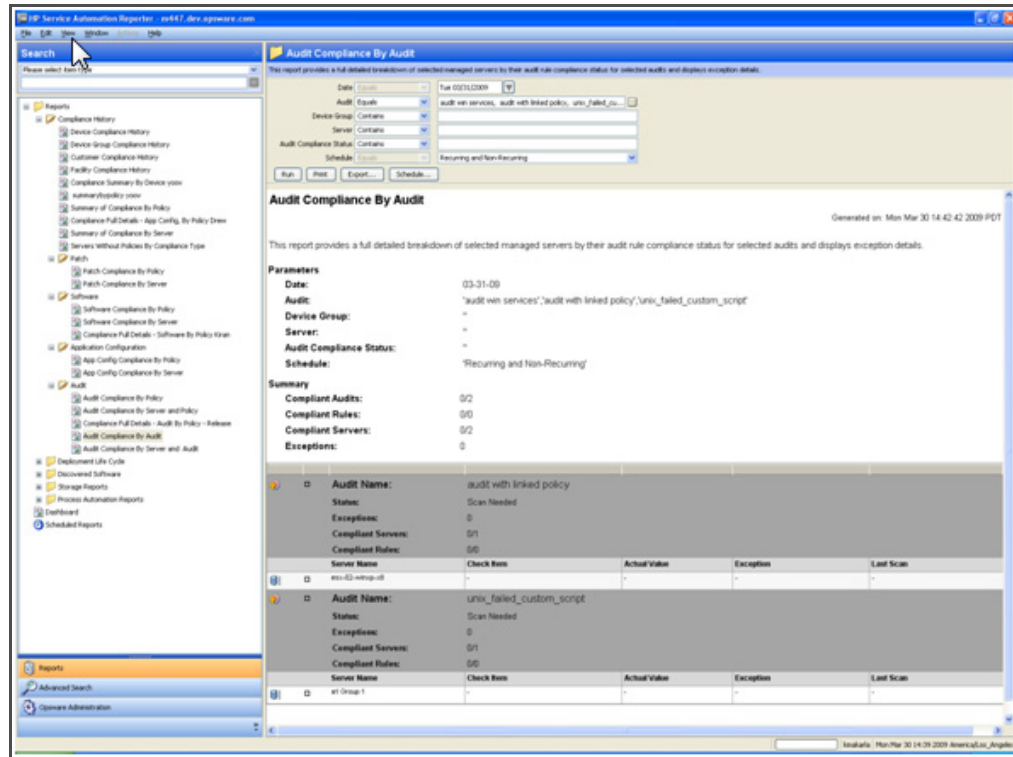
Figure 21 Audit Compliance By Audit - Value-Based Checks
