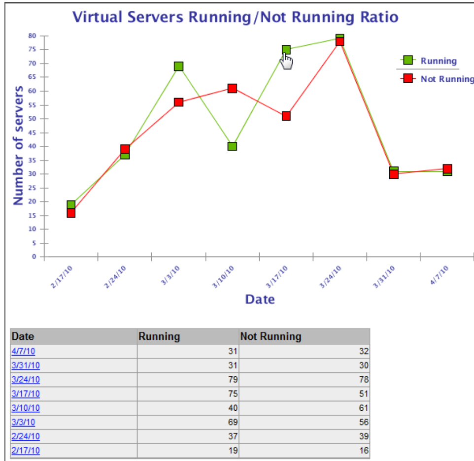
Figure 3 Virtual Servers Running and Not Running
