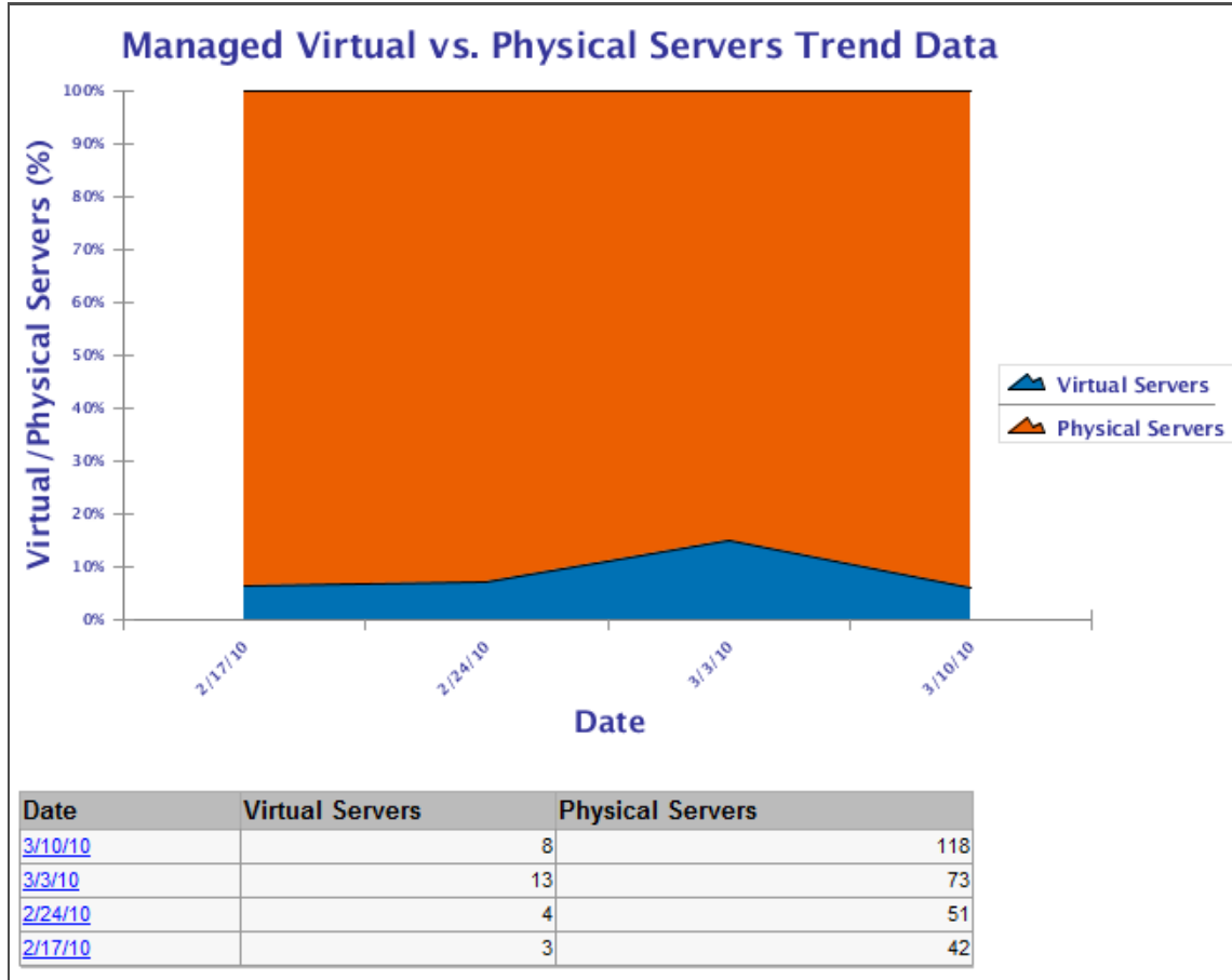
Figure 2 Managed Virtual vs. Physical Servers Trend Data
