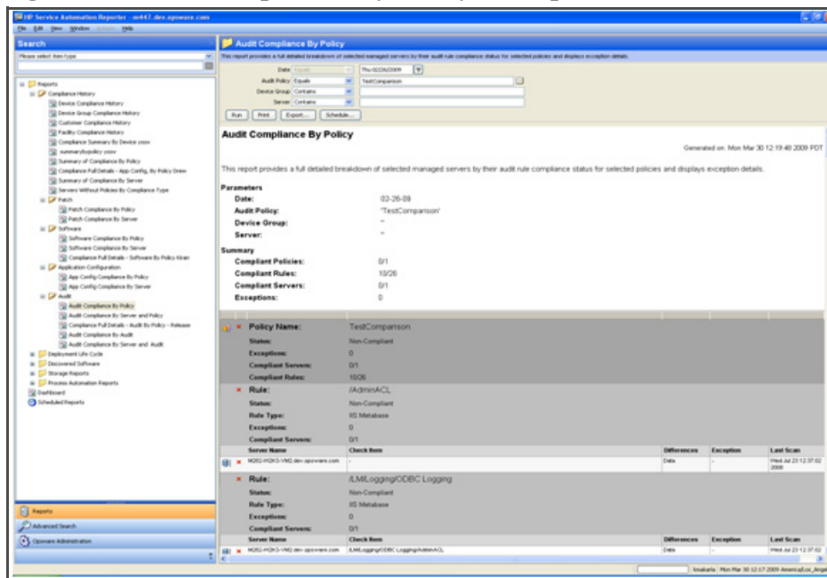
Figure 20 Audit Compliance By Policy - Comparison-Based Checks
