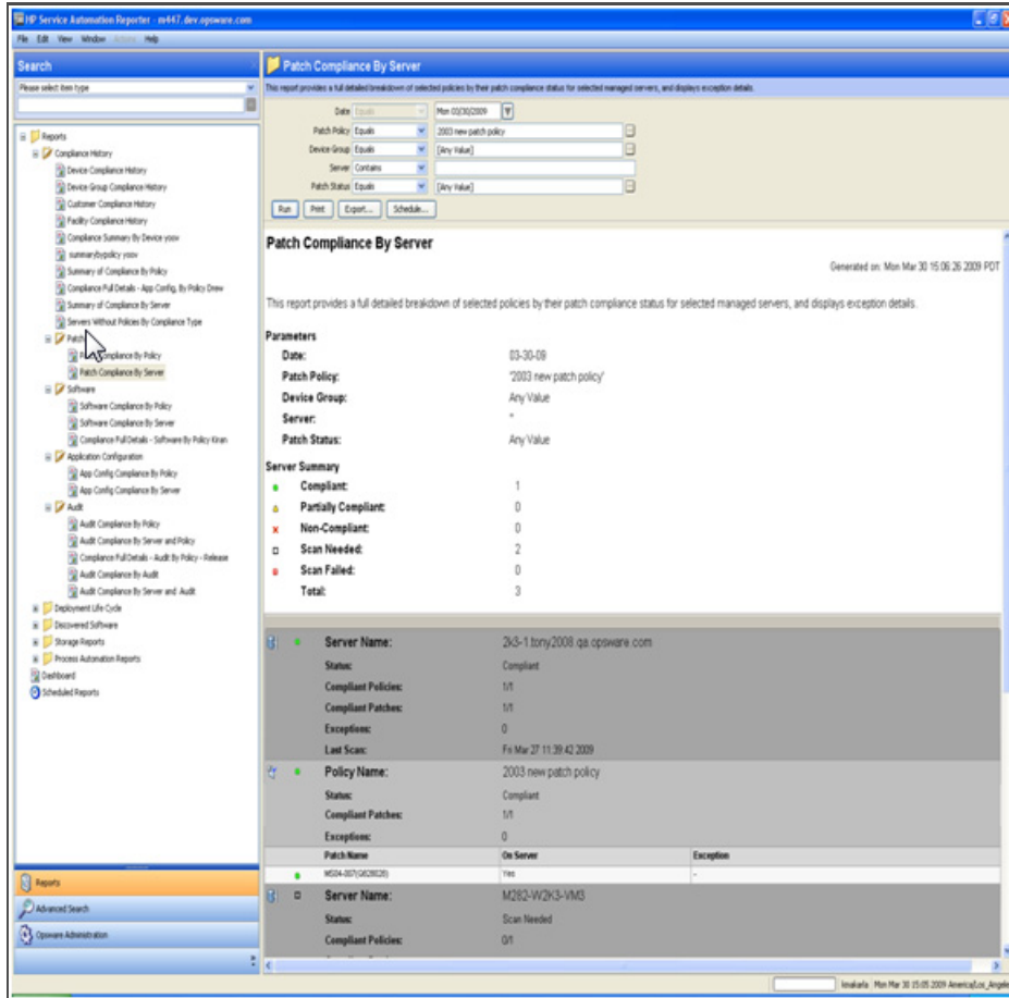
Figure 27 Patch Compliance By Server
