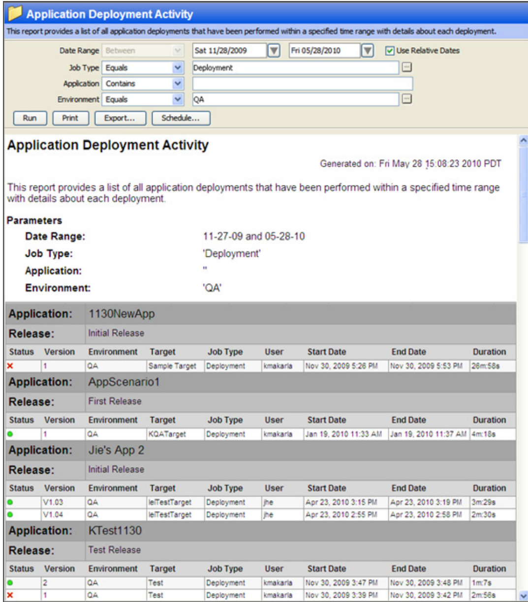
Figure 11 Application Deployment Activity Report
