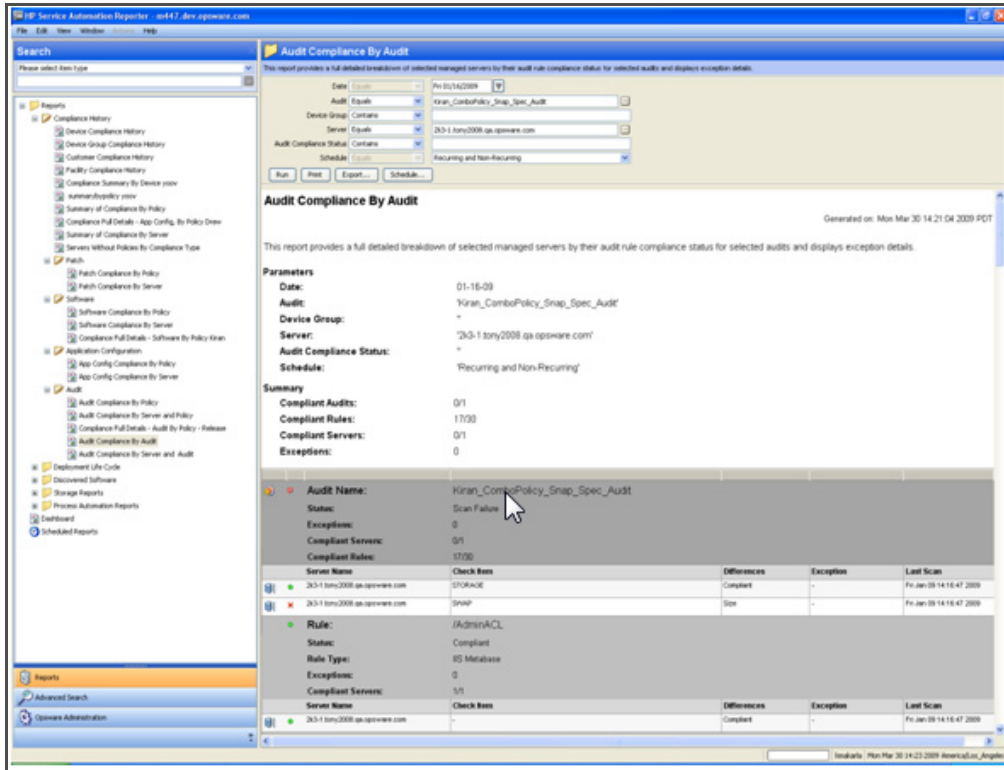
Figure 22 Audit Compliance By Audit - Comparison-Based Checks
