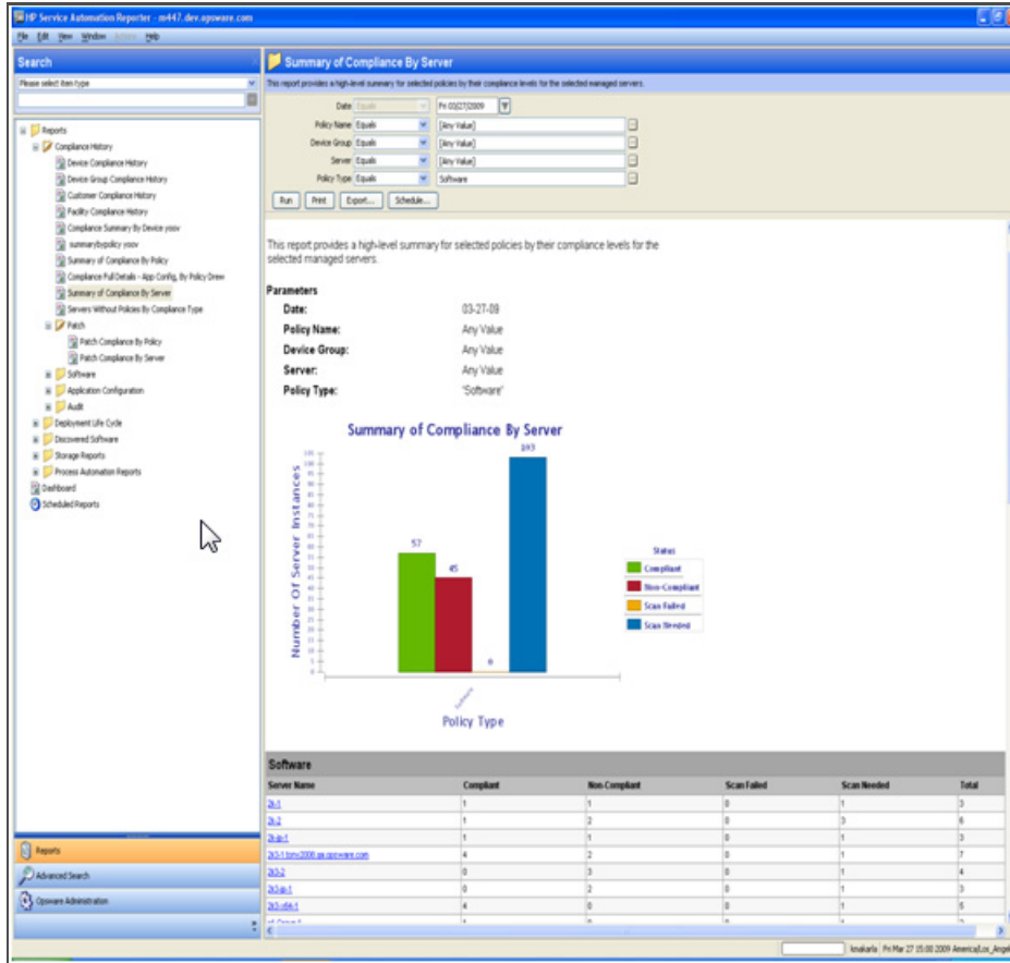
Figure 14 Summary of Compliance By Server
