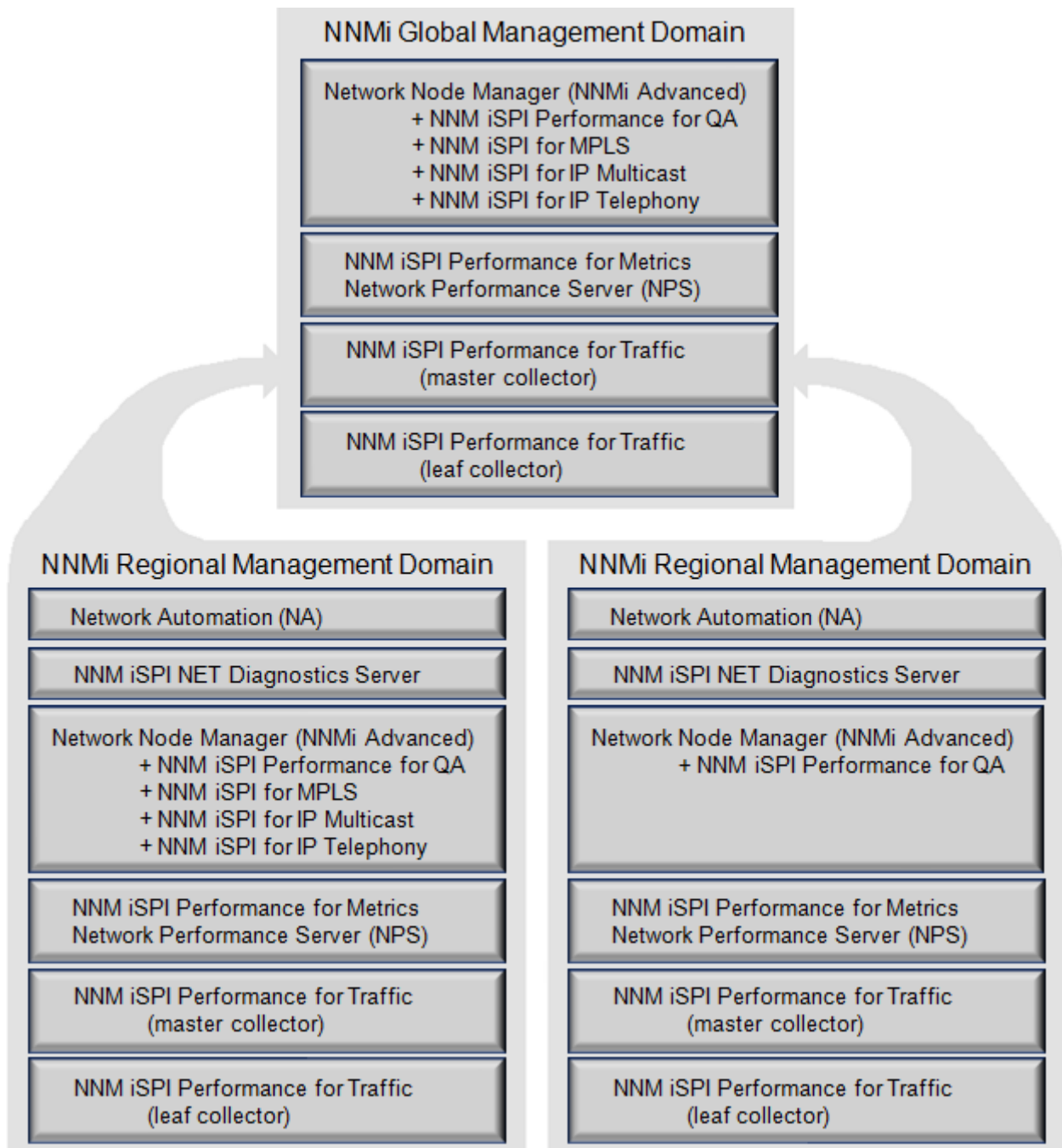
Figure 1 Example Deployment Architecture for One NA Core Associated with Each NNMi Regional Management Server
