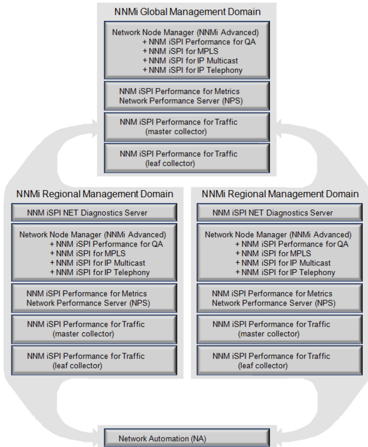
Figure 2 Example Deployment Architecture for One NA Core Associated with Multiple NNMi Regional Management Servers
