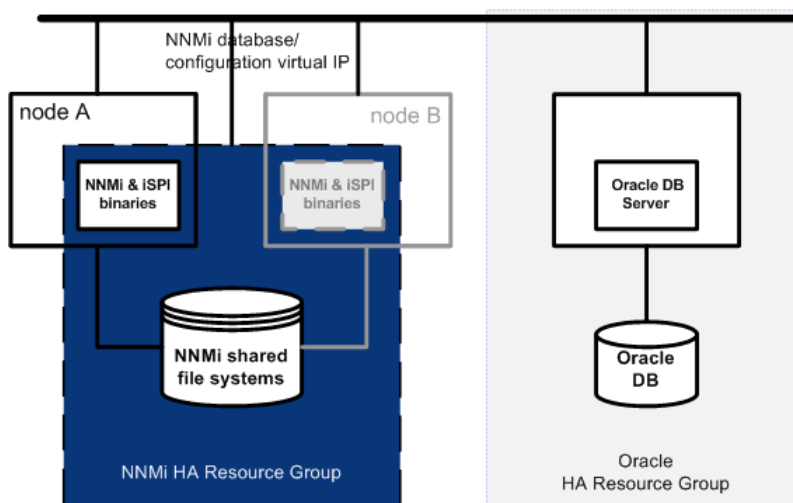
Figure 30 HA for NNMi with an Oracle Database
