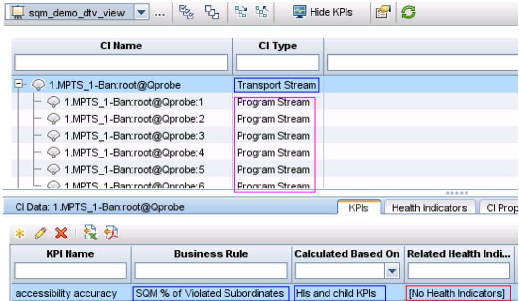
Figure3 KPI propagation result
