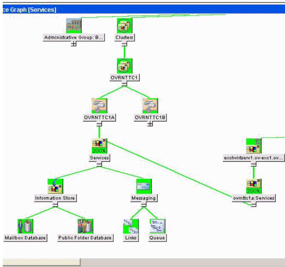
Figure 42 Service Graph of Clustered Nodes
