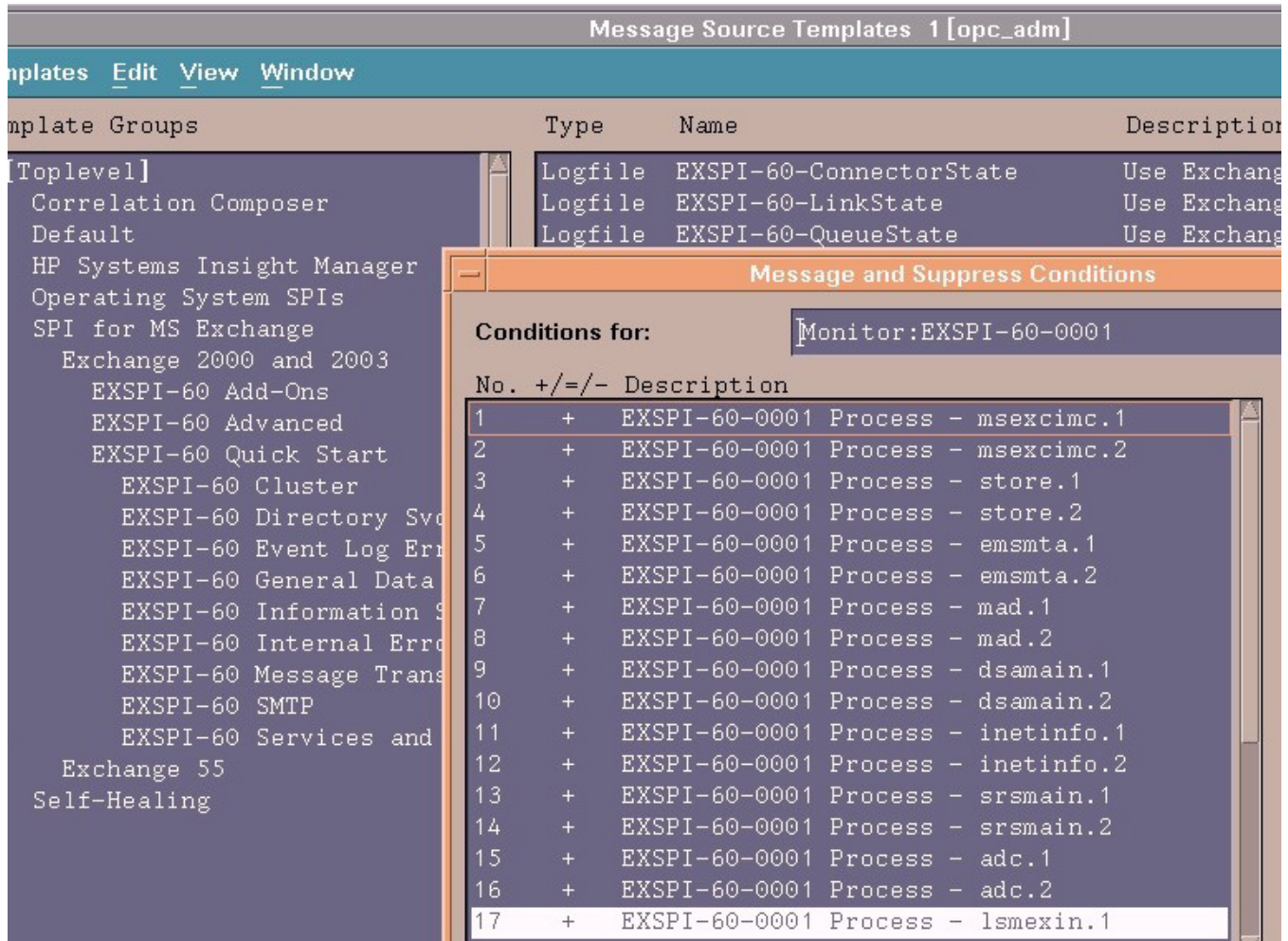
Figure 45 The Message and Suppress Conditions Window
