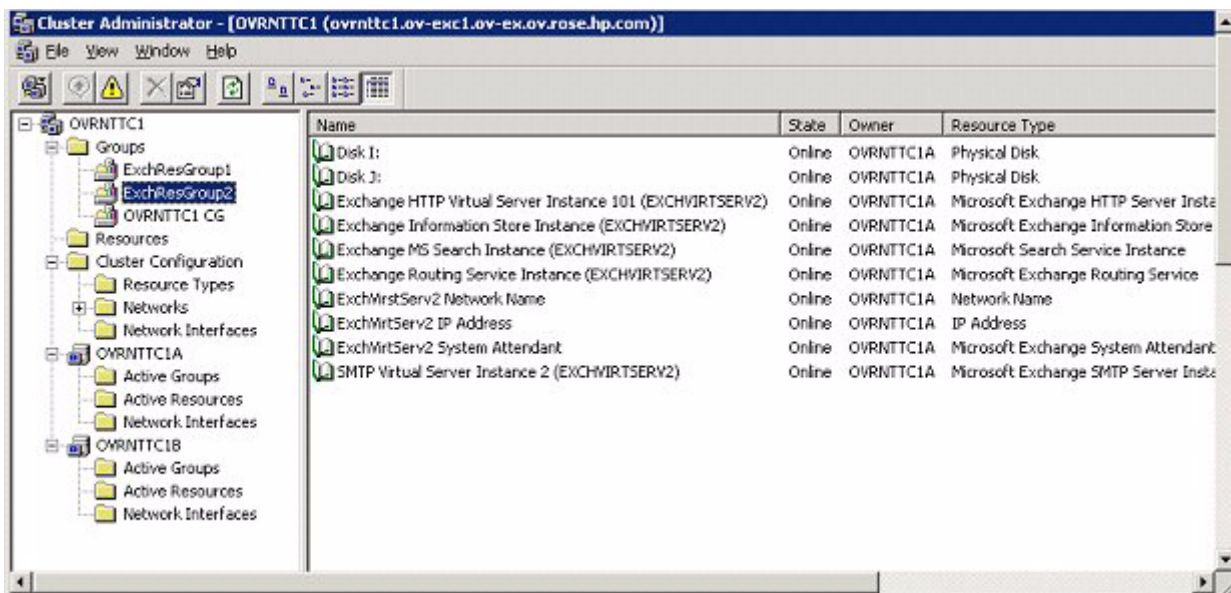
Figure 40 Example Exchange resource group
