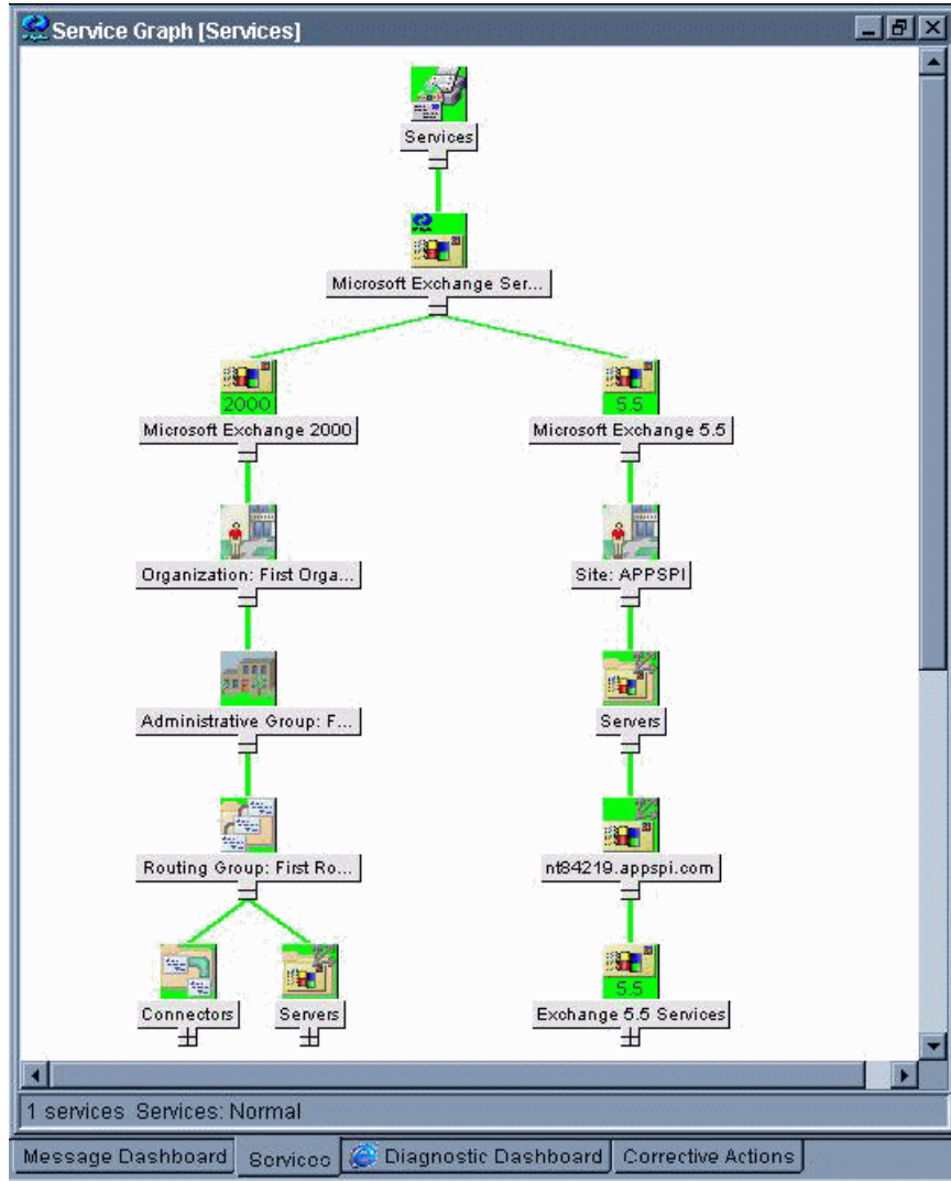
Figure 1 Example Service Map
