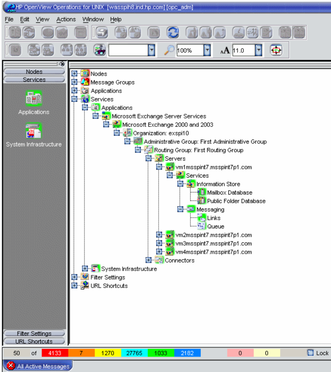
Figure 37 Service Tree View of Service Map
