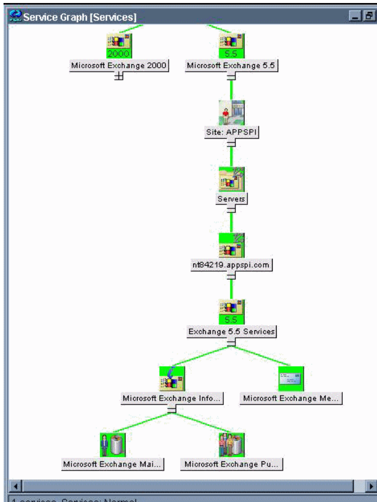
Figure 38 Exchange 5.5 Service Graph
