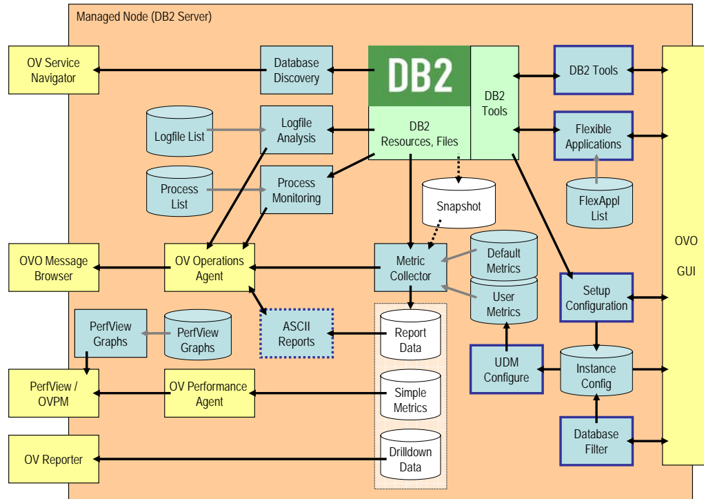
Figure 29: DB2SPI Internal Architecture
