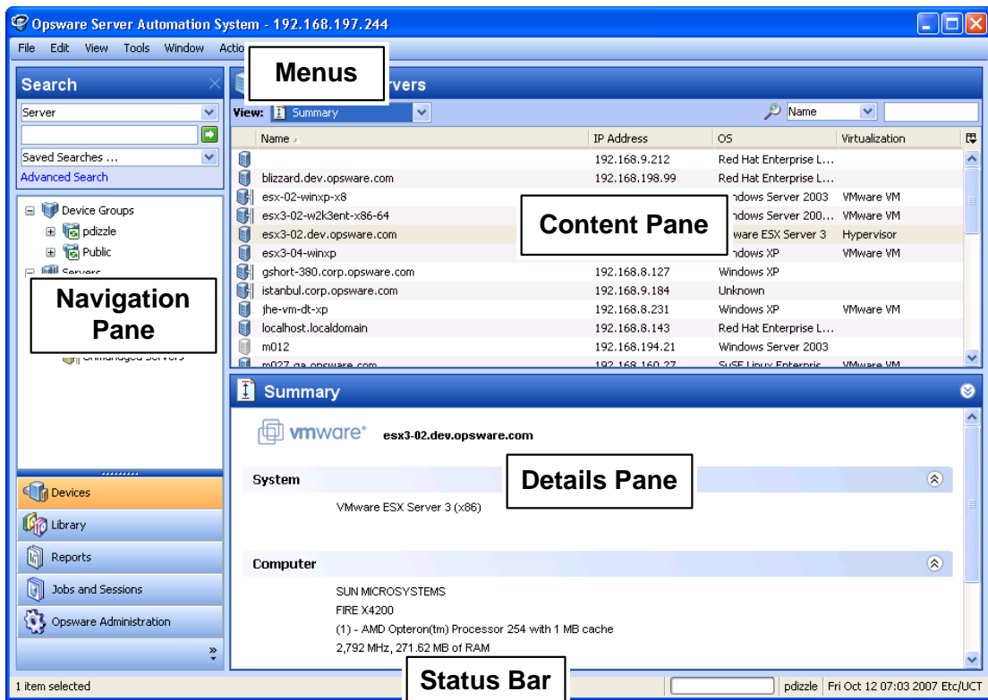
Figure 3-2: SAS Client User Interface
