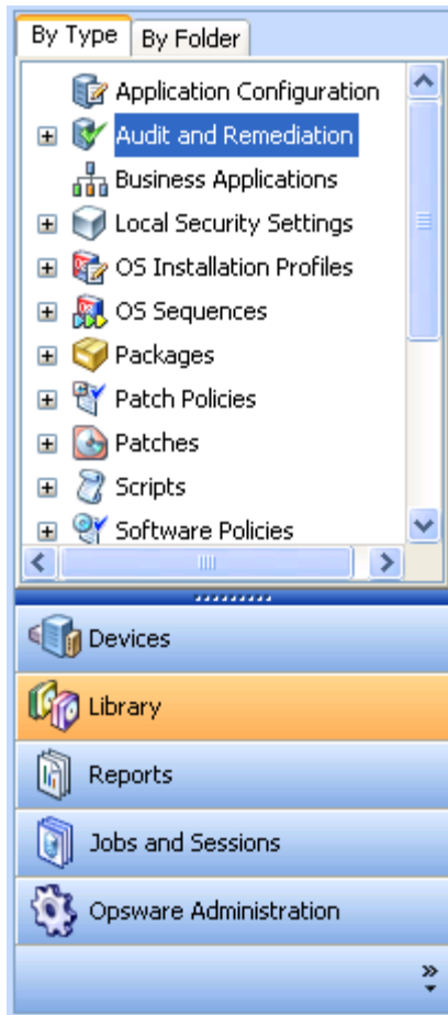
Figure 3-3: Navigation Pane
