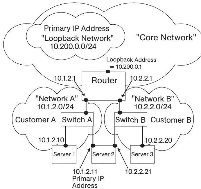
Figure 7-20: Primary IP Addresses in Opsware SAS
