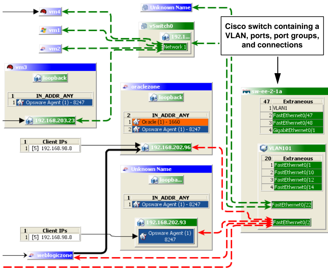
Figure 1-11: Network Map
