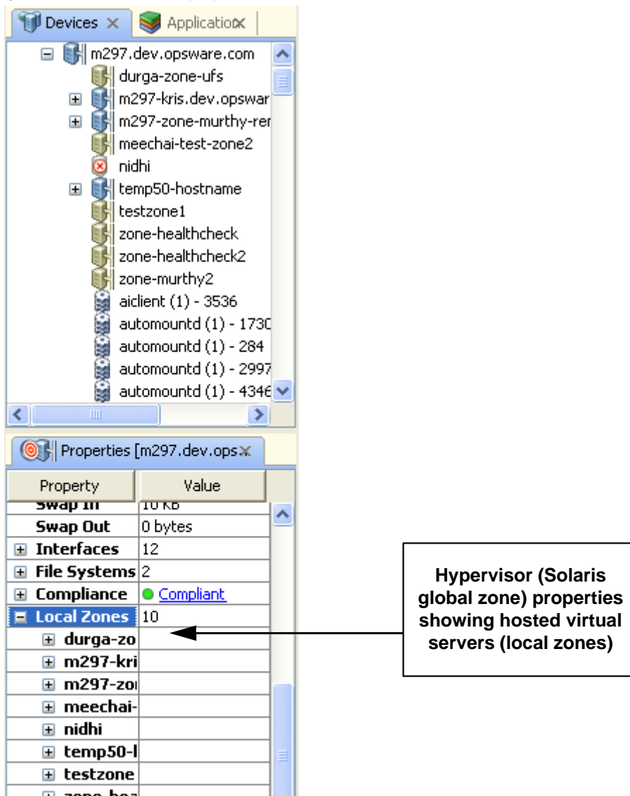
Figure 1-15: Virtual Server properties
