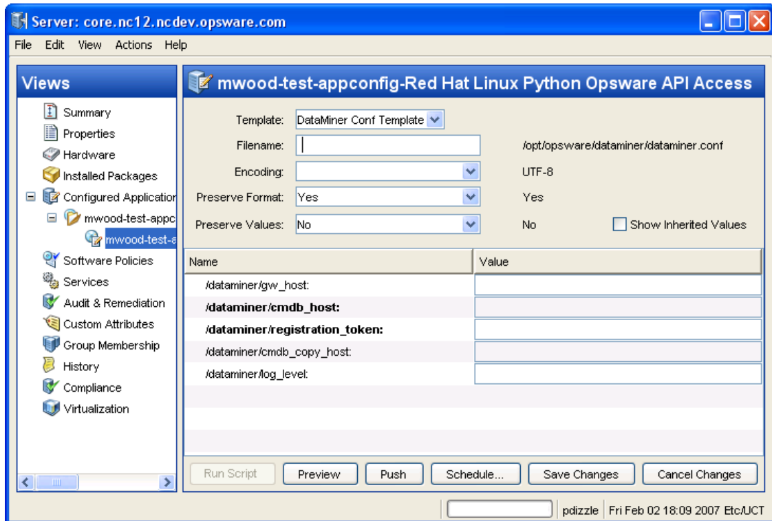
Figure 8-3: Value Set Editor in the Server Explorer
