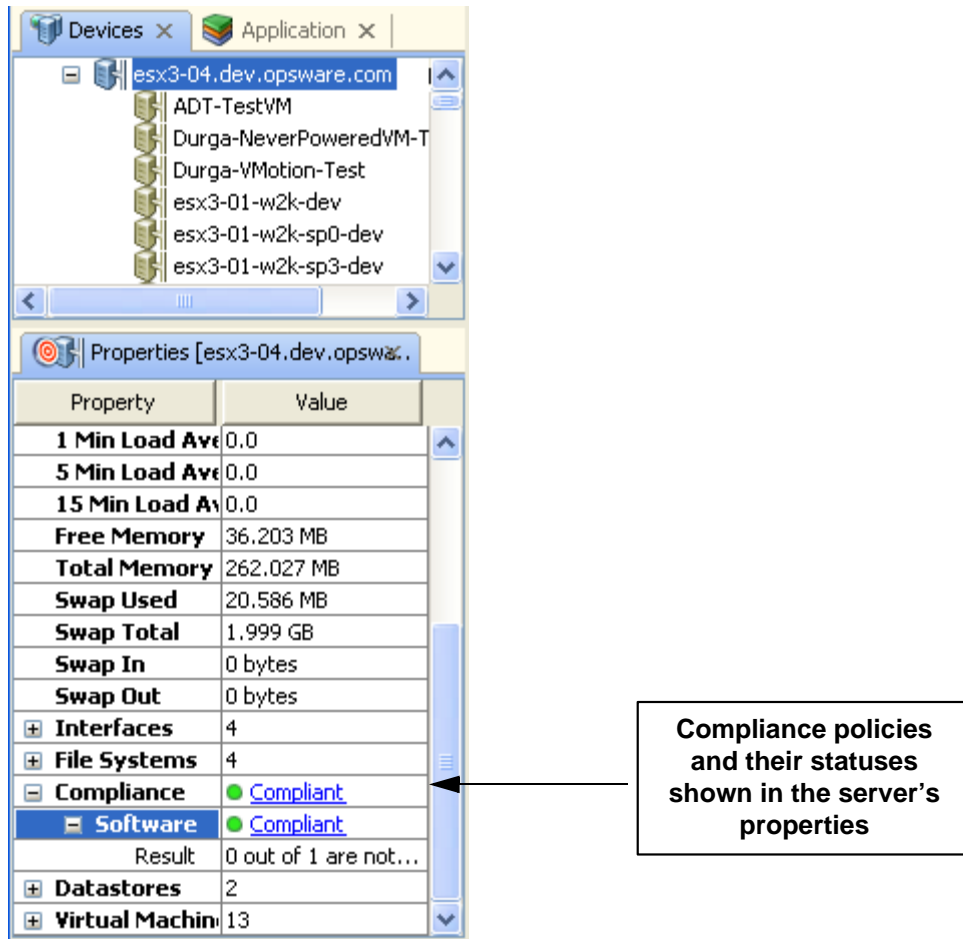
Figure 1-14: Server properties compliance Information
