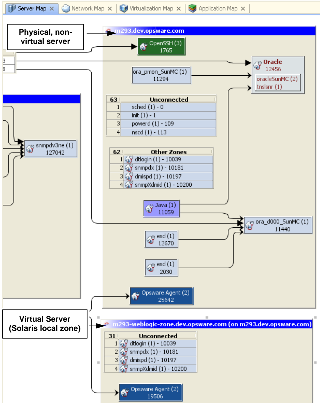
Figure 1-9: Server Map
