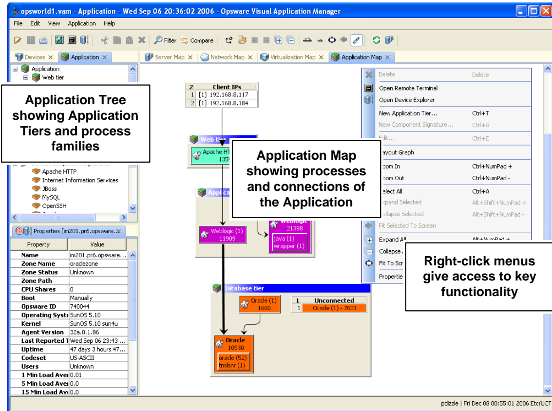
Figure 1-2: Opware Visual Application Manager User Interface
