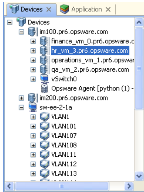
Figure 1-5: Device Tree
