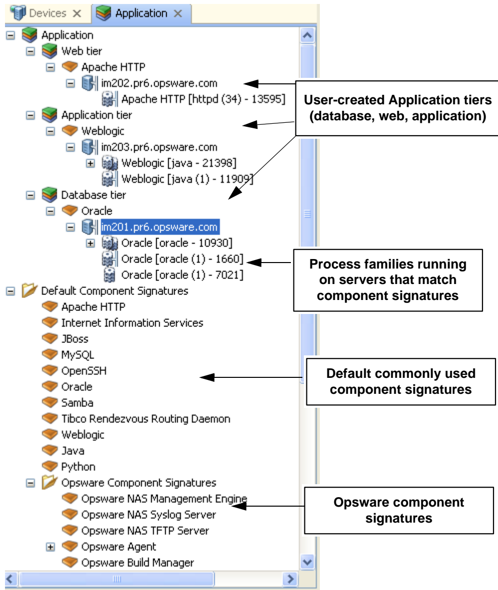
Figure 1-4: Application Tree
