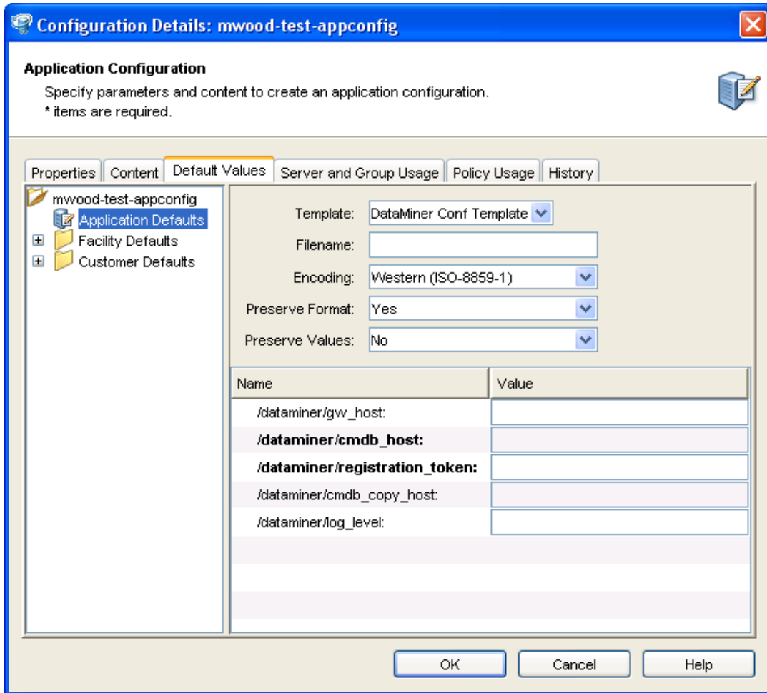
Figure 8-2: Application Configuration Default Values
