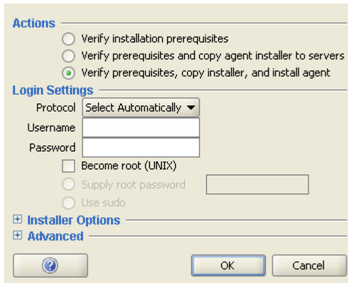
Figure 4-7: Deploy Agents
