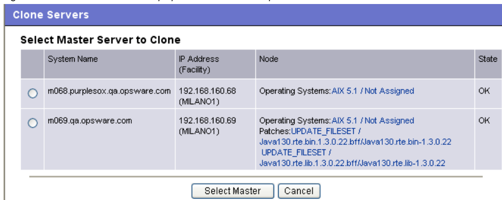
Figure 7-12: Clone Servers Popup Window in the Opware Command Center
