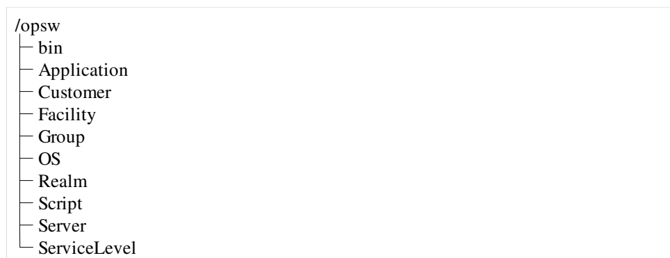
Figure 10-2: opsw Directory
