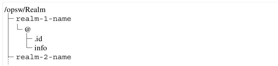
Figure 10-10: Realm Directory
