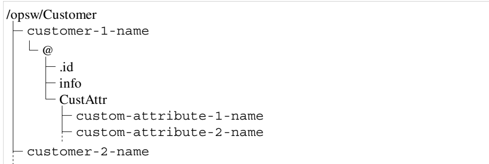
Figure 10-8: Customer Directory
