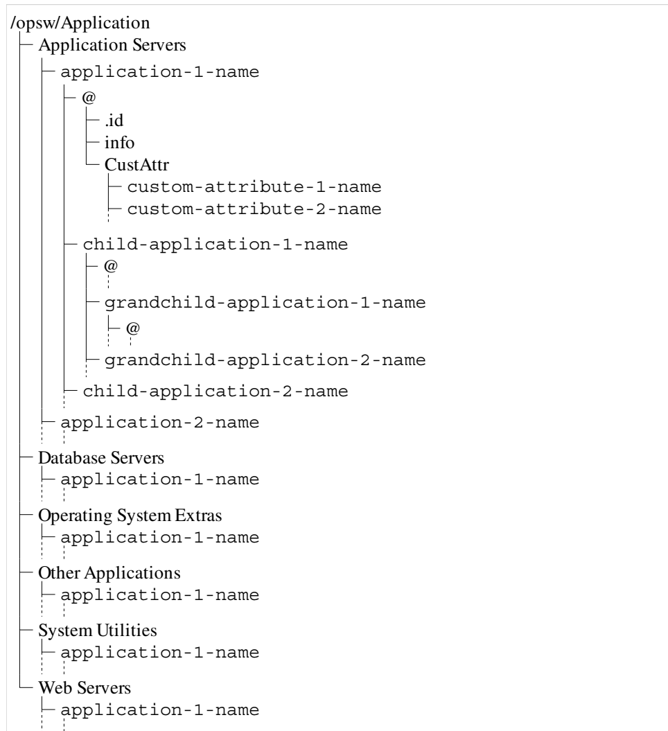
Figure 10-7: Application Directory
