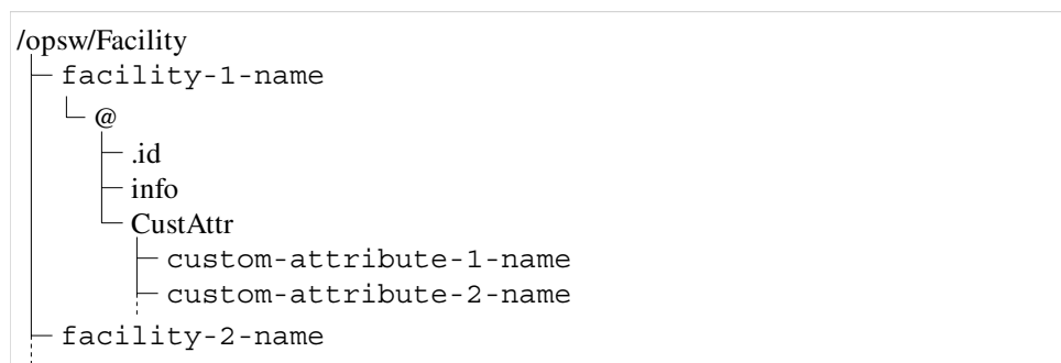
Figure 10-3: Facility Directory
