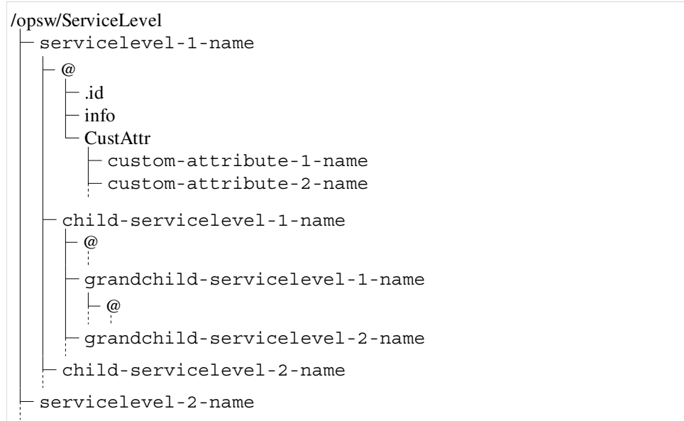
Figure 10-11: ServiceLevel Directory
