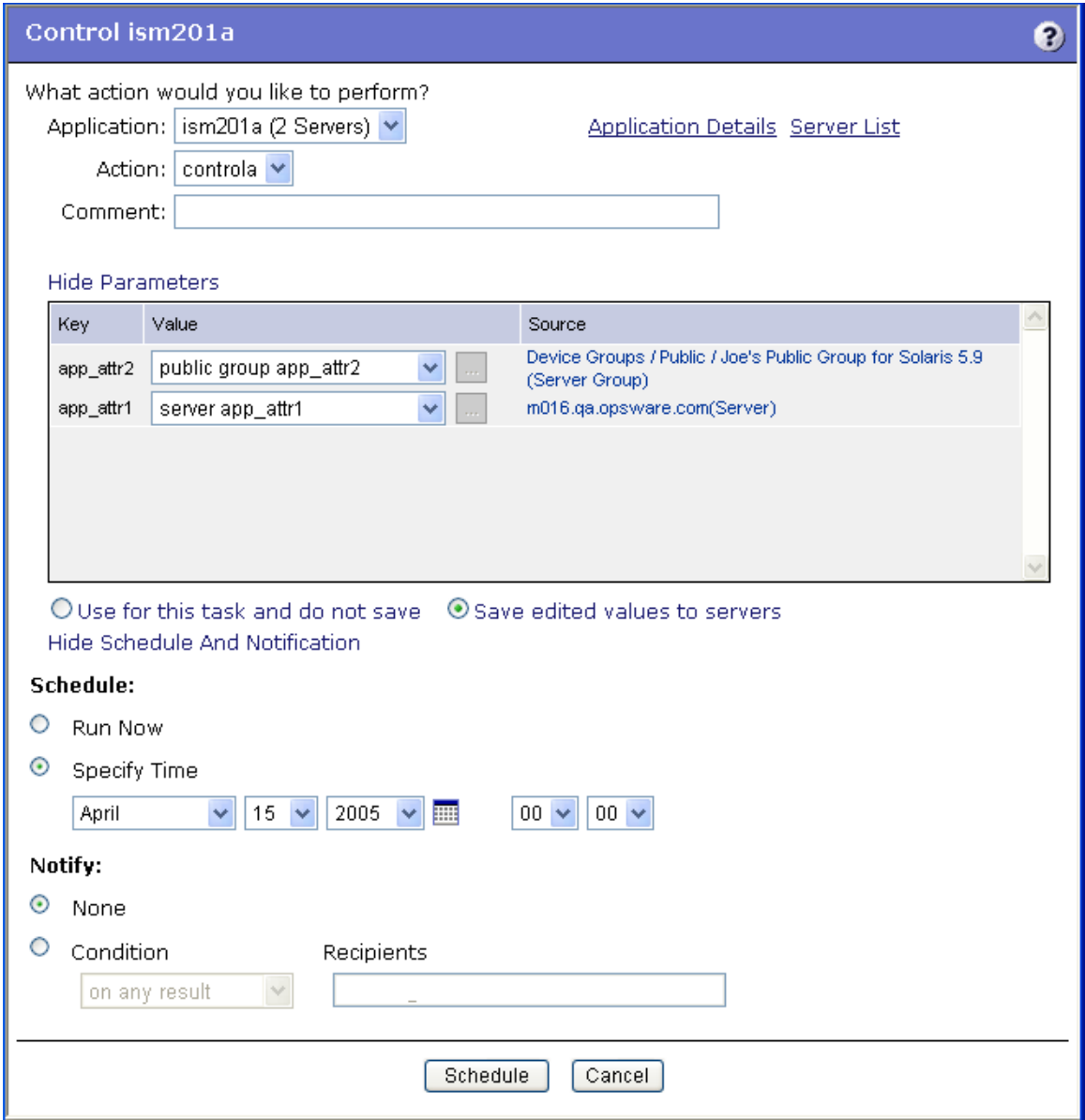
Figure 11-15: Control Window Showing Parameters, Schedule, and Notification
