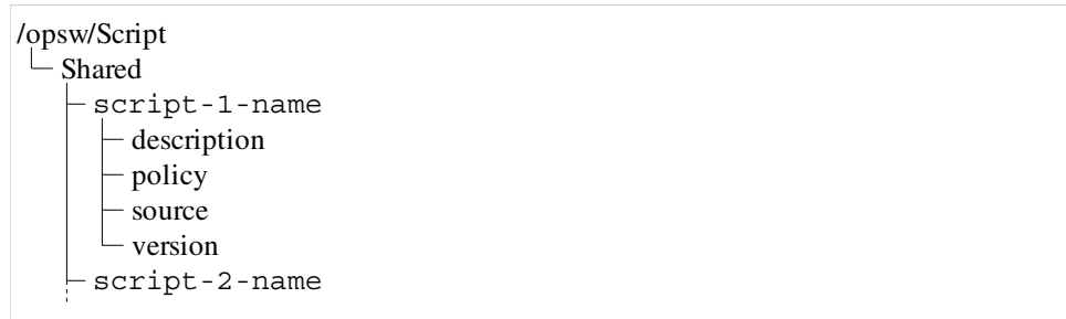
Figure 10-6: Script Directory
