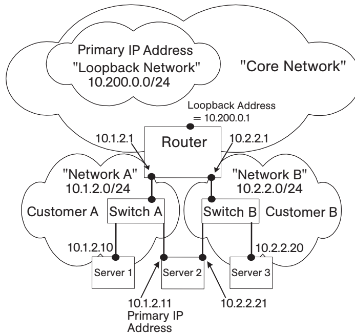
Figure 4-21: Primary IP Addresses in Opware SAS
