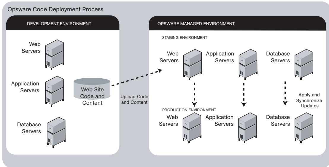
Figure 17-1: Typical Code and Content Update in the Opware Managed Environment
