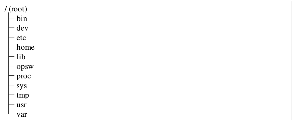
Figure 10-1: root Directory
