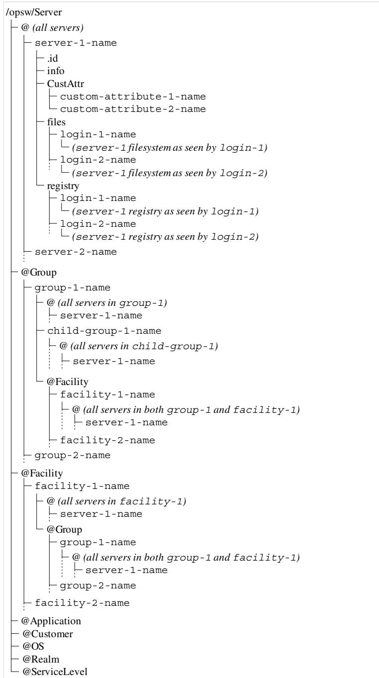
Figure 10-5: Server Directory
