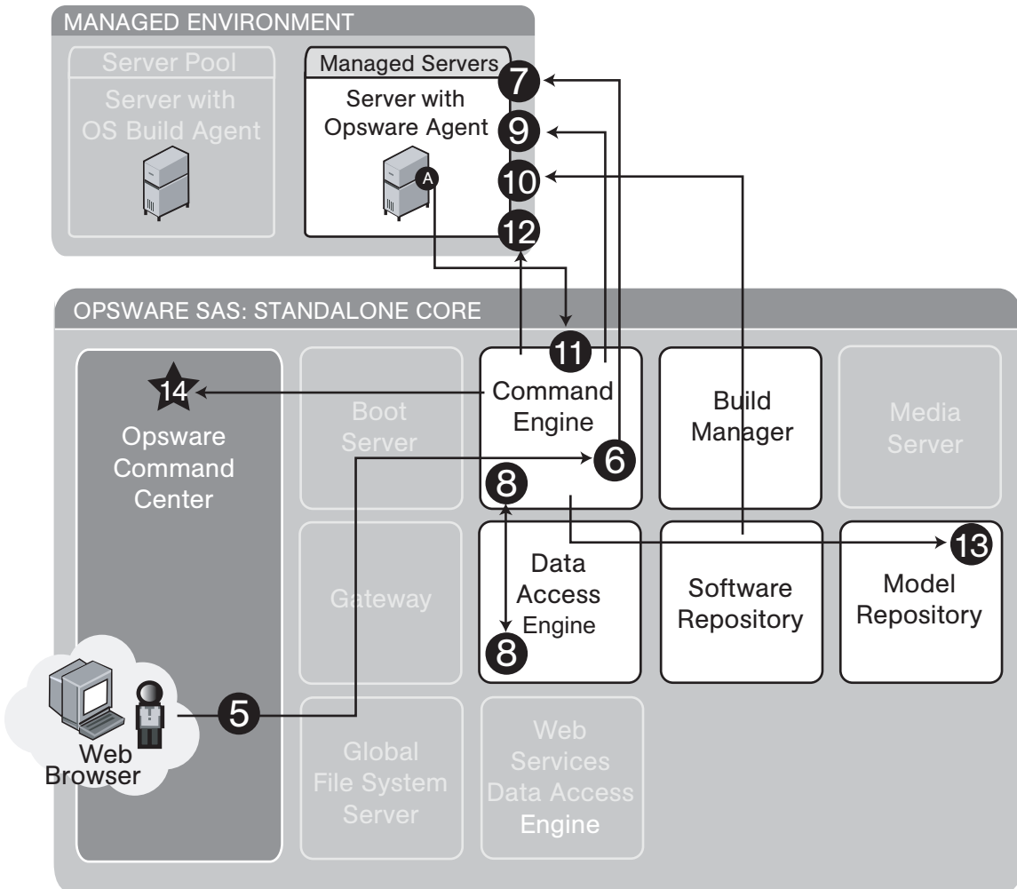
Figure 1-10: Software Provisioning Step 2: Software Installation and/or Removal Through Reconcile
