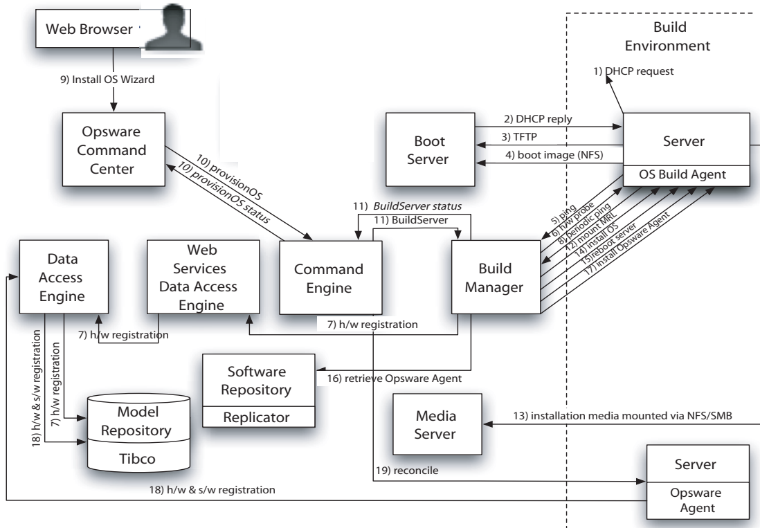
Figure 1-4: OS Provisioning Feature Interaction
