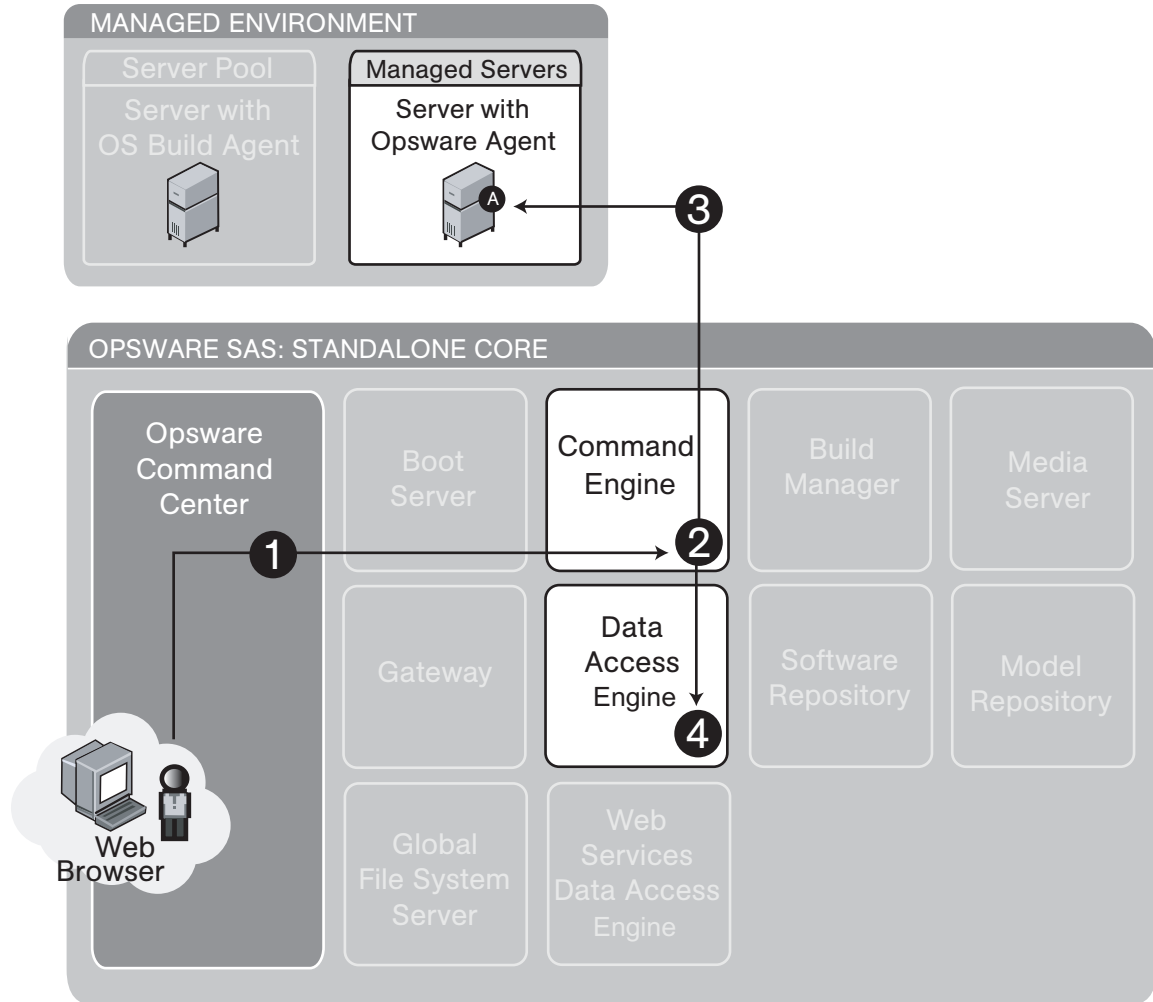
Figure 1-9: Software Provisioning Step 1: Preview Reconcile
