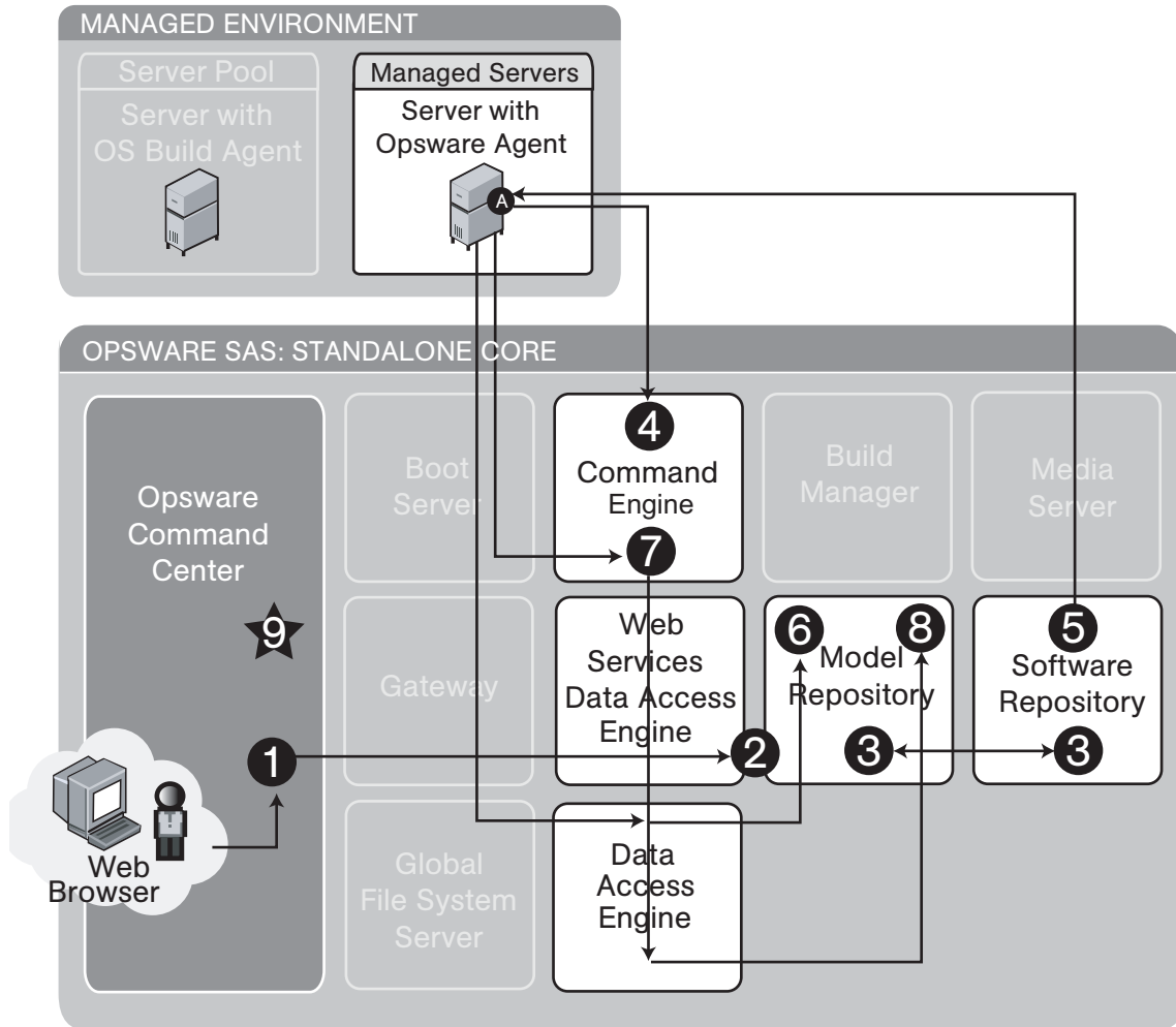
Figure 1-6 illustrates the install patch process:
