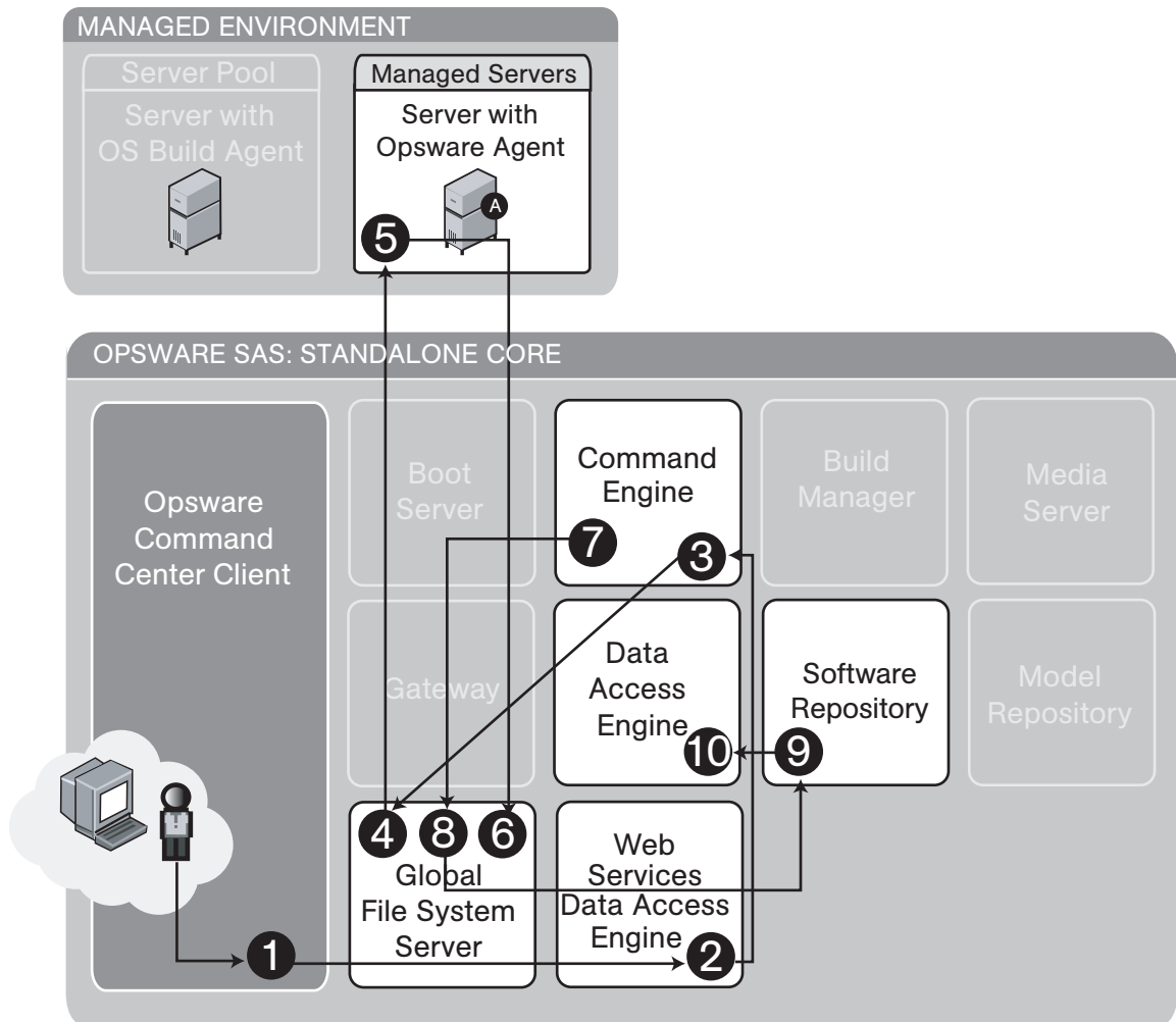
Figure 1-19: Component Interaction of Auditing a Server
