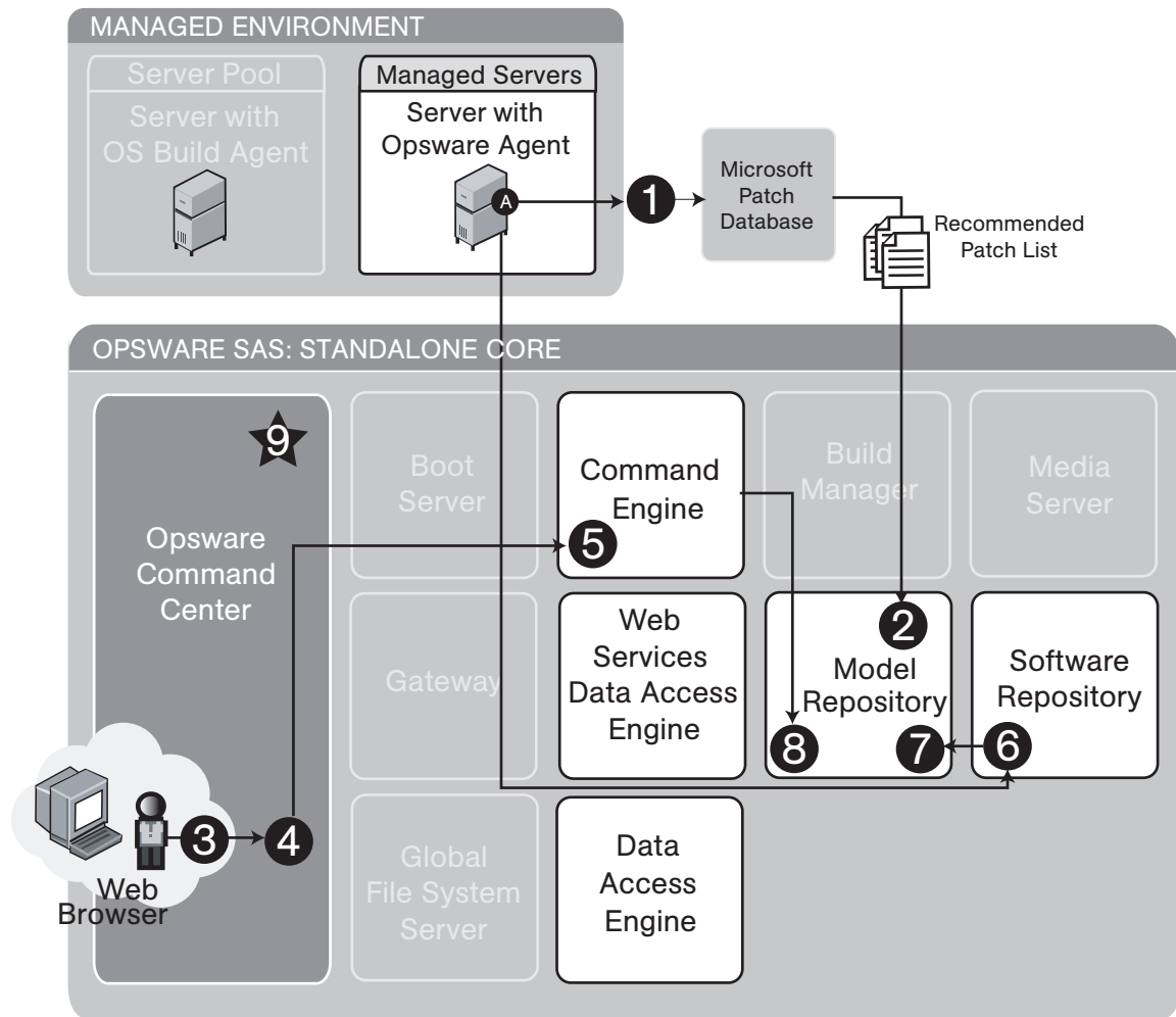
Figure 1-8 illustrates the Microsoft patch update process:
