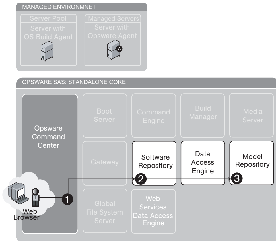
Figure 1-5: Patch Management Feature: Upload Patch
