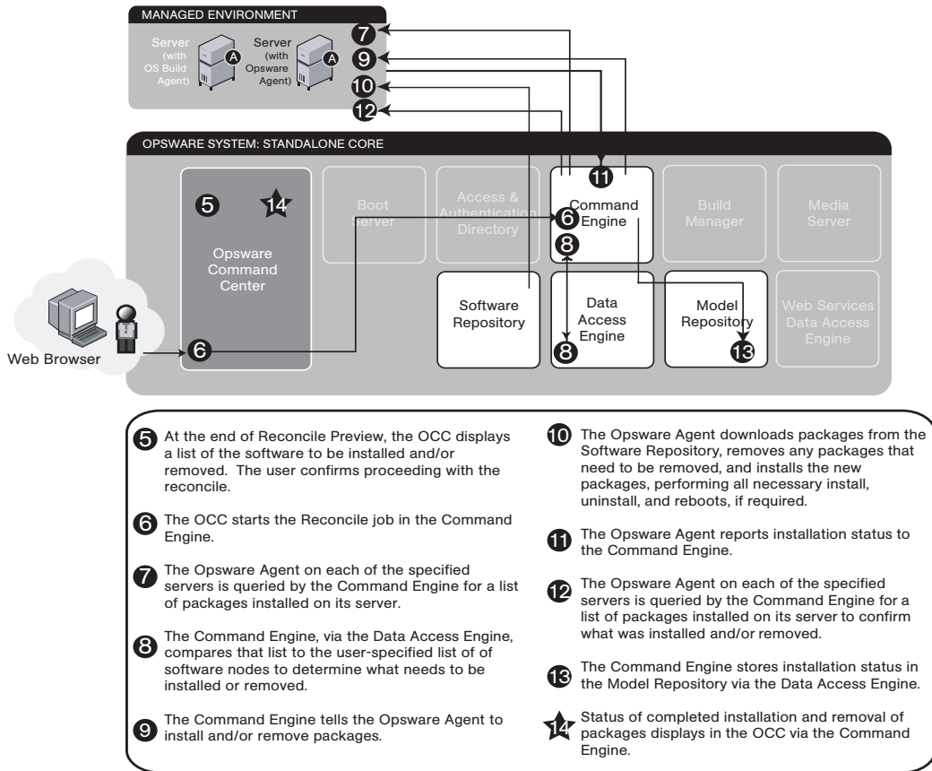
Figure 1-10: Application Provisioning Step 2: Software Installation and/or Removal Through Reconcile
