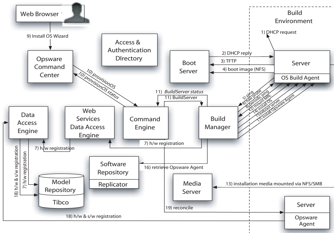
Figure 1-4: OS Provisioning Subsystem Interaction
