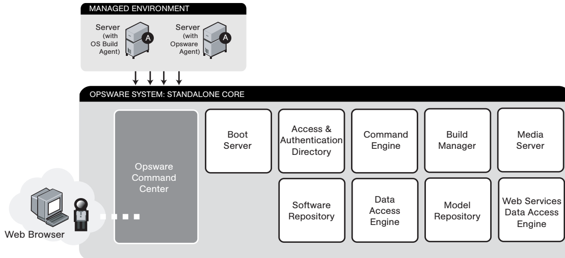
Figure 1-3: General Overview of All Components
