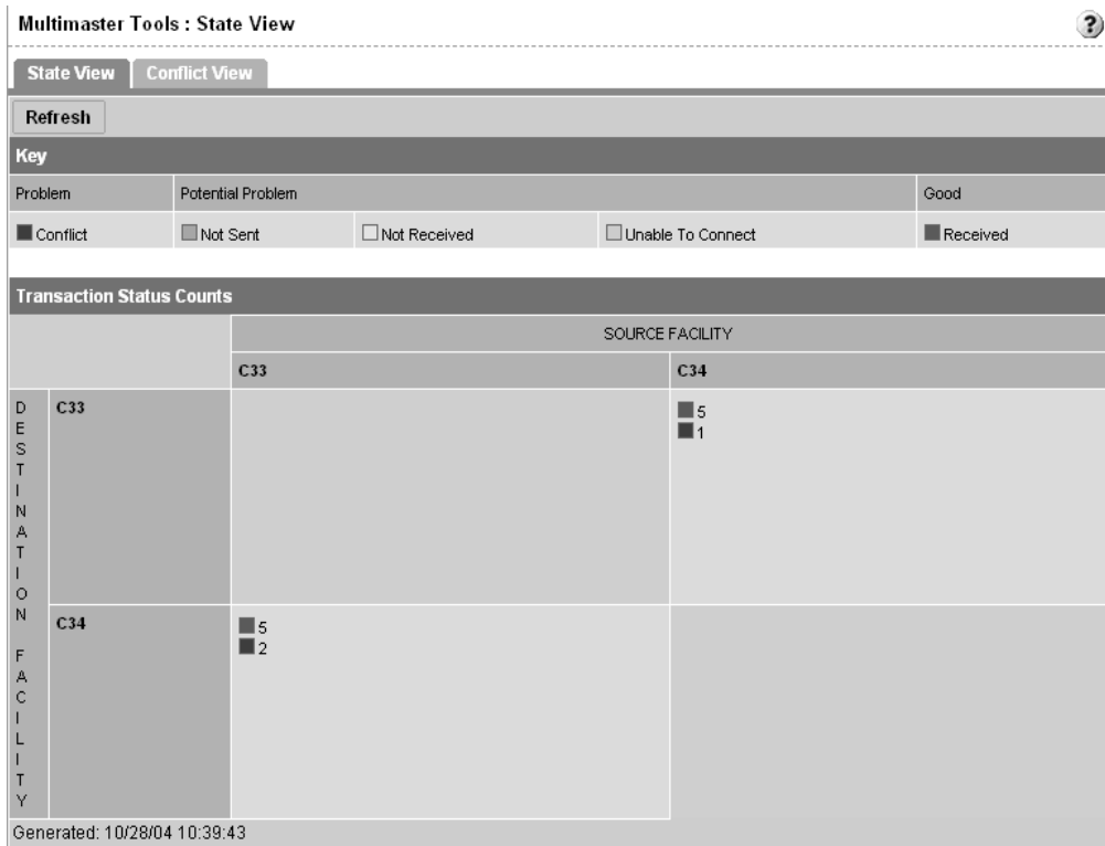
Figure 2-30: Transaction Table That Shows Conflicts
