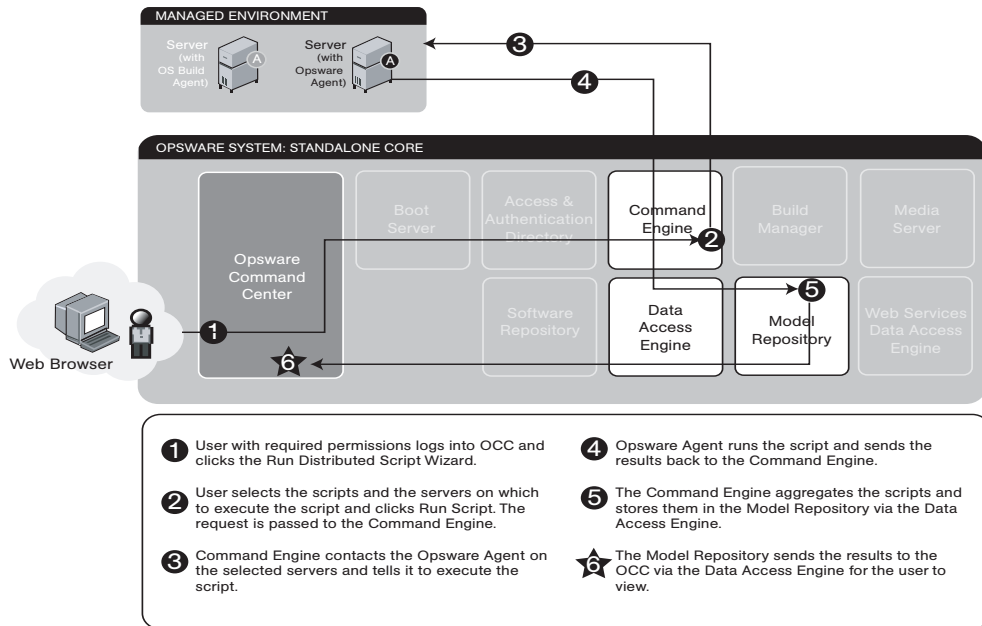
Figure 1-13: Scripting Subsystem: Execute Scrip
