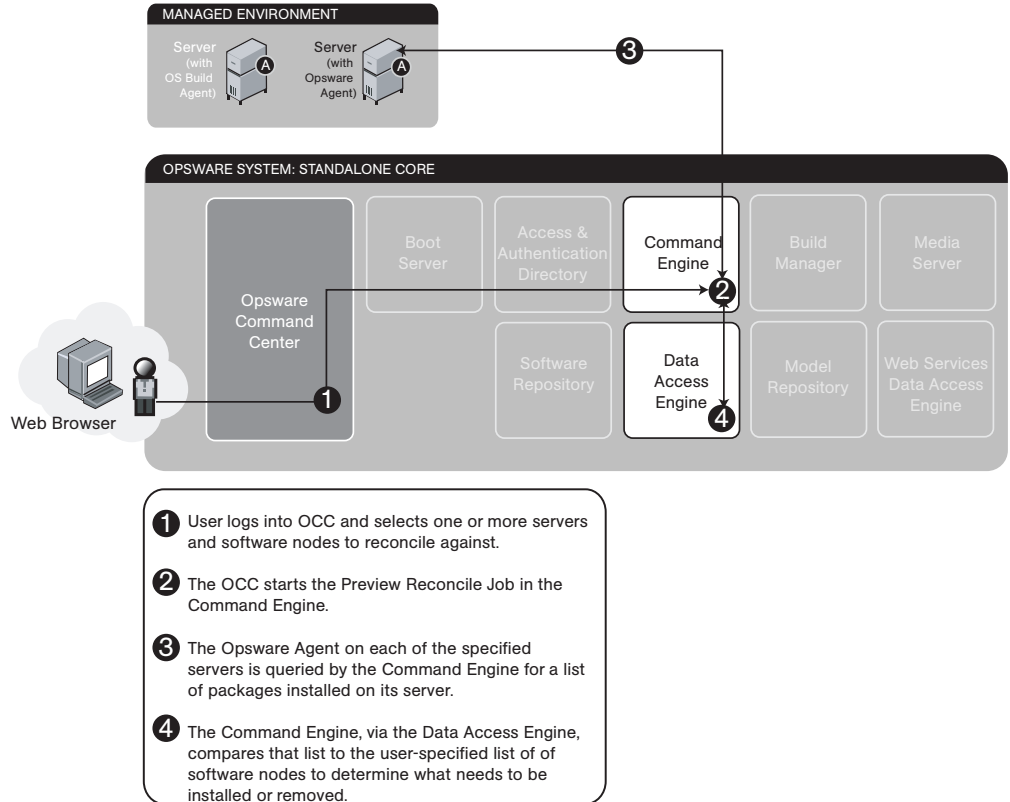
Figure 1-9: Application Provisioning Step 1: Preview Reconcile
