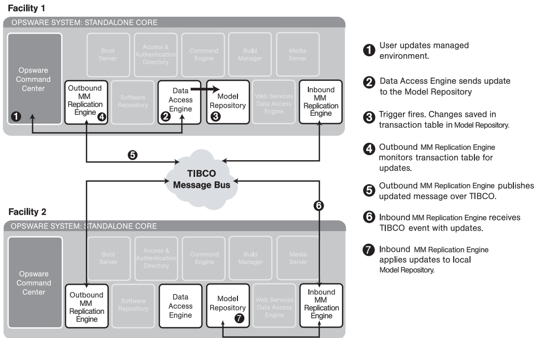
Figure 1-15: Interaction Between Components in Multiple Facilities
