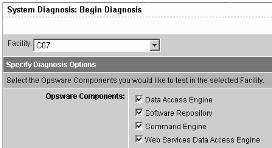
Figure 3-1: System Diagnosis Page That Shows Opware Components Selected for Testing on the Indicated Facility
