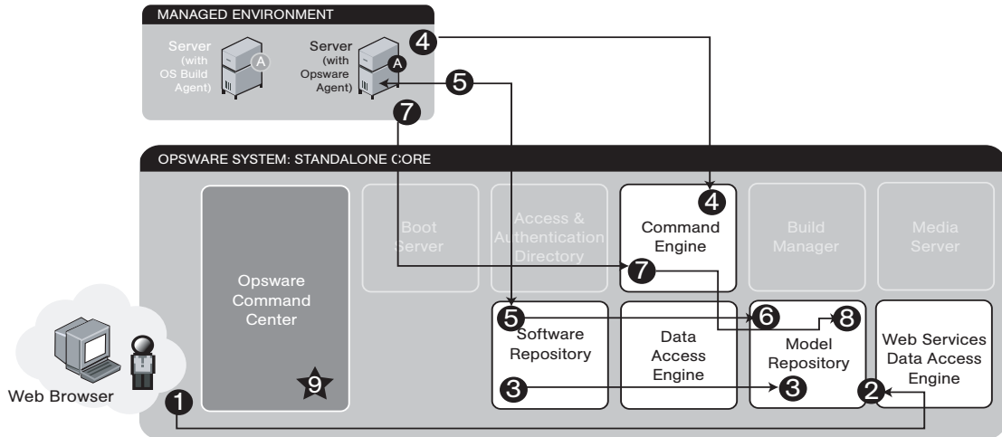
Figure 1-6: Patch Management Subsystem: Install Patch
