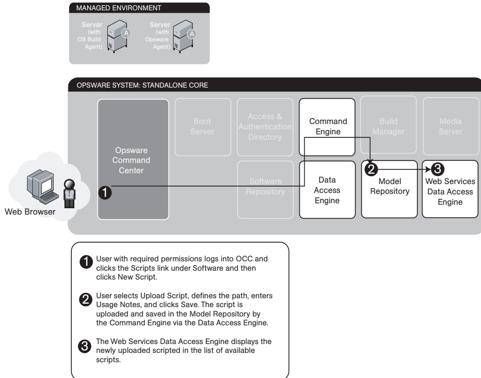
Figure 1-12: Scripting Subsystem: Upload Script
