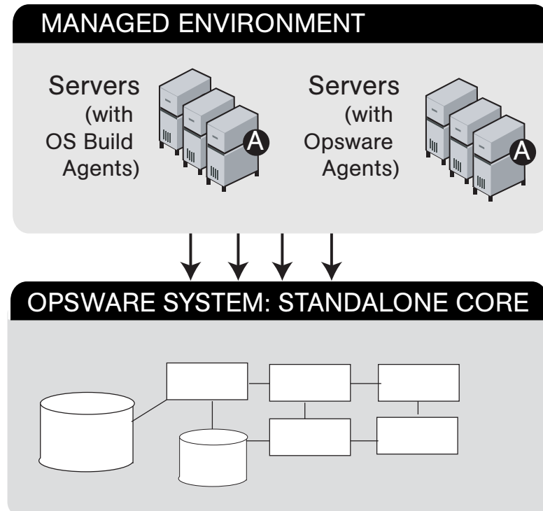
Figure 1-1: Opware System Environment
