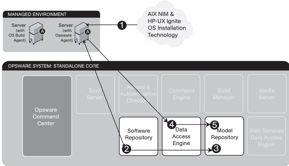
Figure 1-14: Opware Integration with AIX and HP-UX OS Installation Technology
