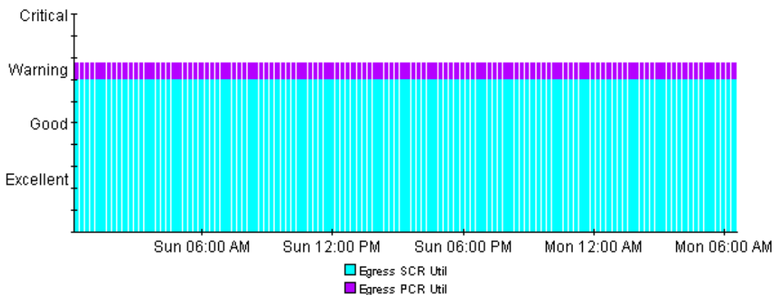
PVC Egress Grade of Service ATMSwitch1: 50-0-34 Sun, Dec 2 12:14 AM - Mon, Dec 3 6:29 AM
