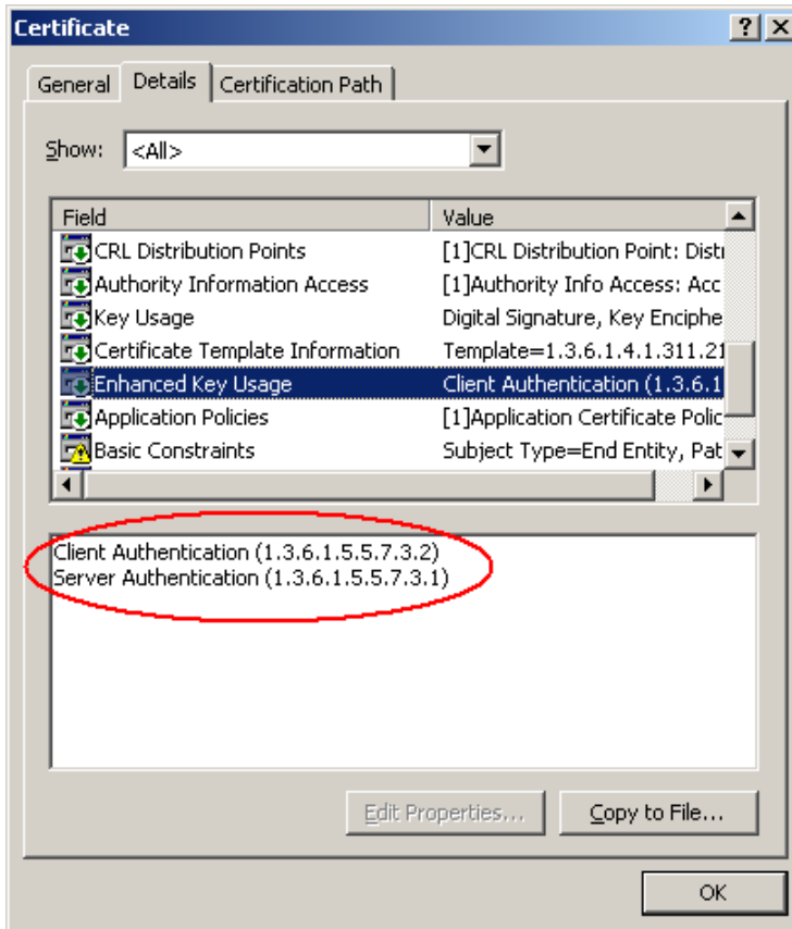
Figure 2 - response.cer editor
