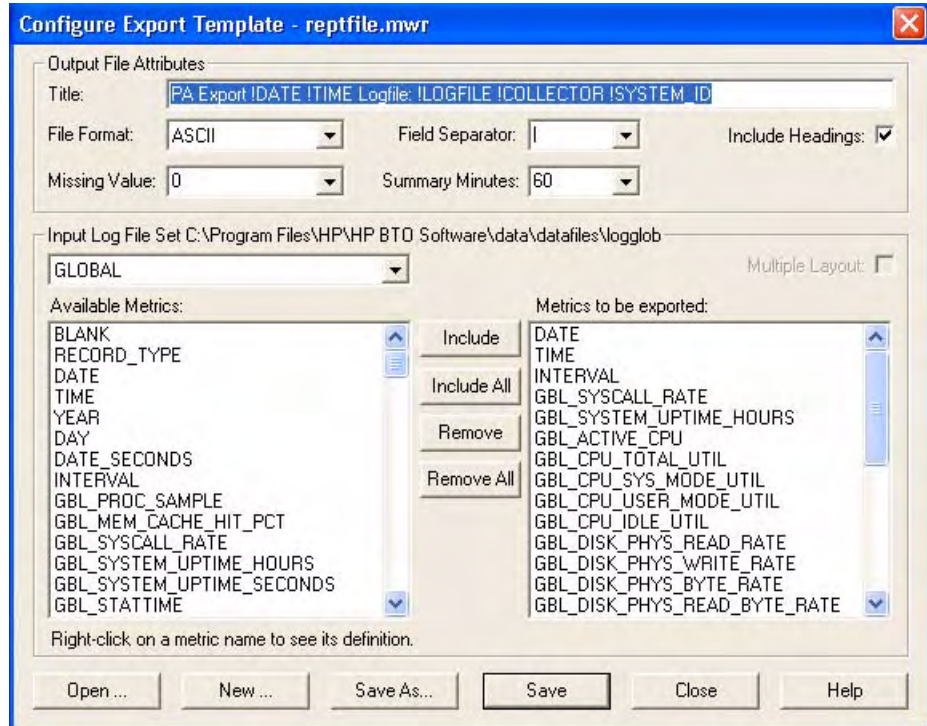
Figure 7 Configure Export Template Dialog Box
