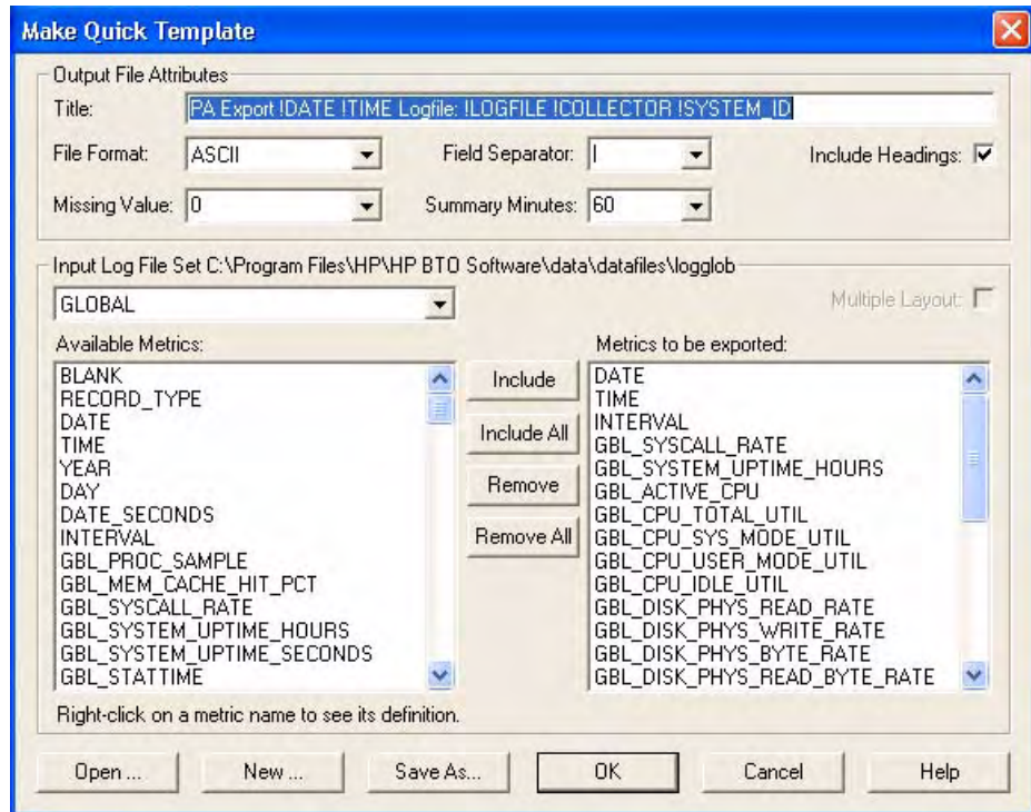
Figure 6 Make Quick Template Dialog Box
