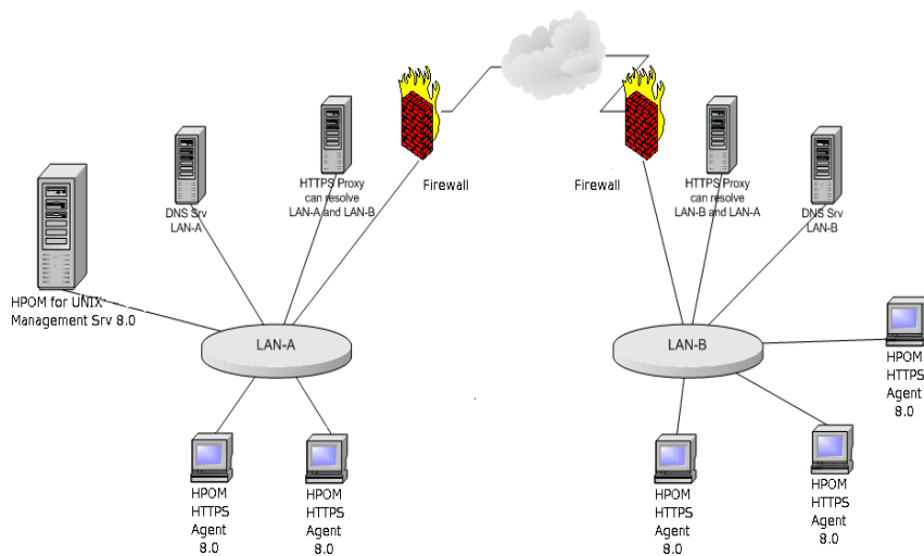
Figure 8-1 HTTP Proxy Schematic
