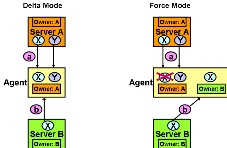
Figure 10-1 Policy Handling Between Multiple Configuration Servers, Server A Has a Different Owner than Server B.
