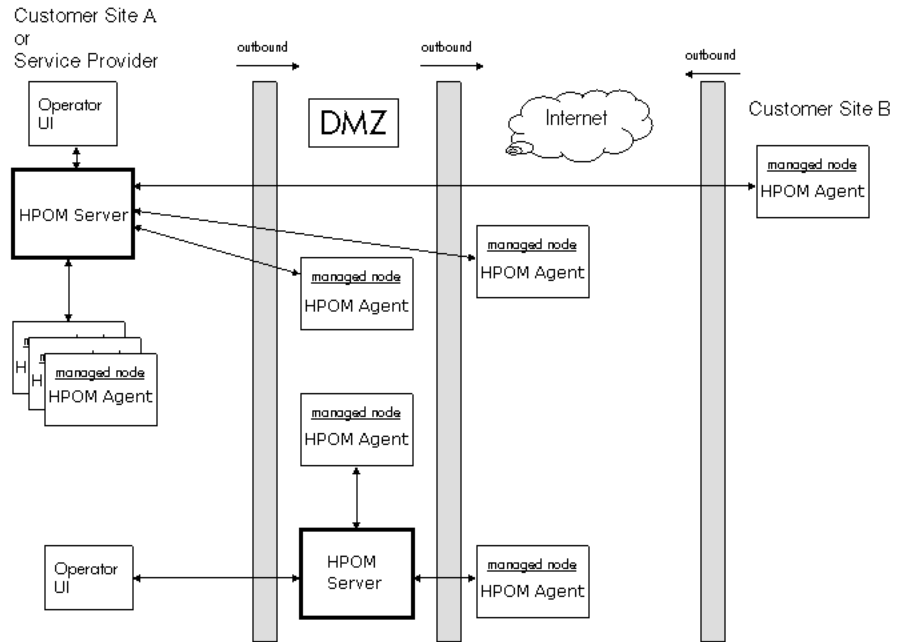
Figure 1-1 A Typical HPOM Managed Environment
