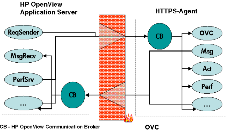
Figure 2-2 Crossing a Firewall with HTTPS Communication
