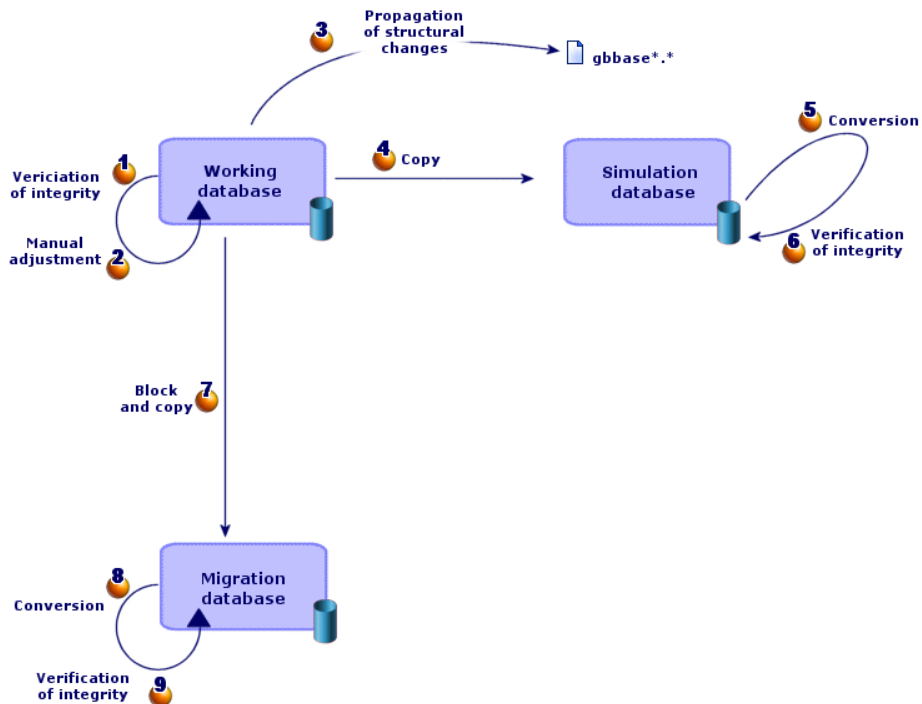
Figure 2.2. Conversion - process to convert AssetCenter versions 4.2.x and 4.3.x
