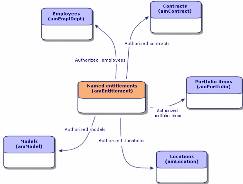
Figure 4.3. Software - tables involved in named entitlements
