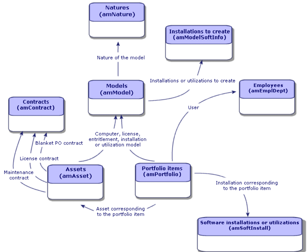
Figure 4.1. Software - Physical data model
