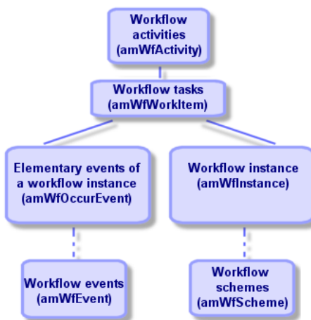
Figure 8.4. Workflow - main tables involved in a workflow instance being executed
