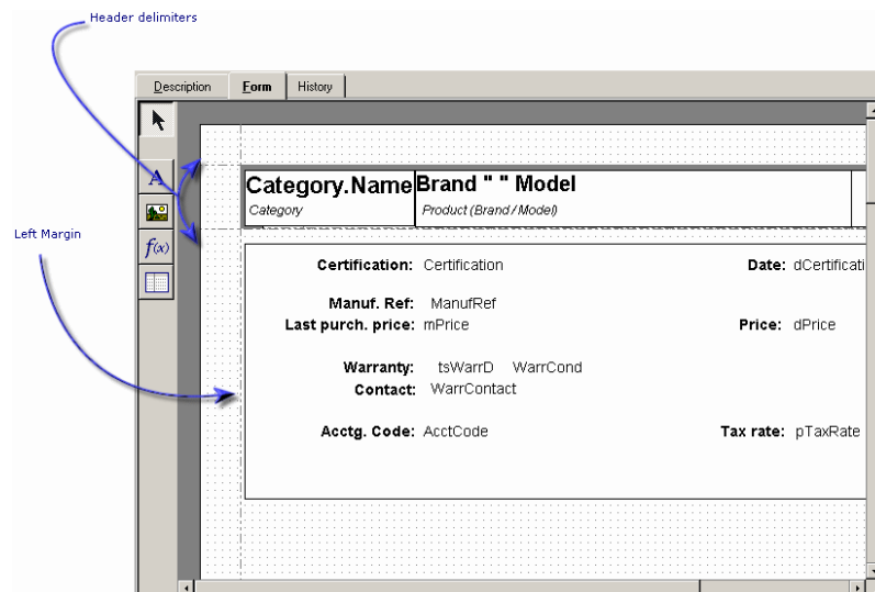
Figure 4.1. Forms - header zone
