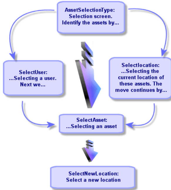
Figure 14.3. Wizard - organization example
