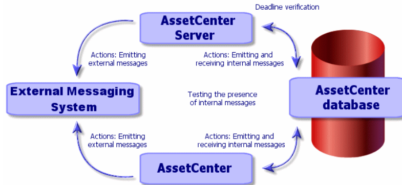
Figure 7.1. Messaging - overview
