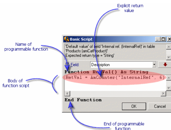
Figure 10.1. Script - builder
