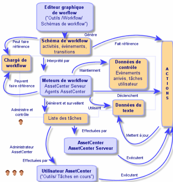
Figure 8.2. Workflow AssetCenter - vue générale
