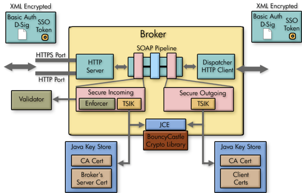
Figure 10-1: Message Level Security
