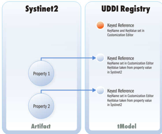
Figure 7. Registry Mapping
