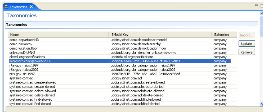
Figure 35. Taxonomies Editor
