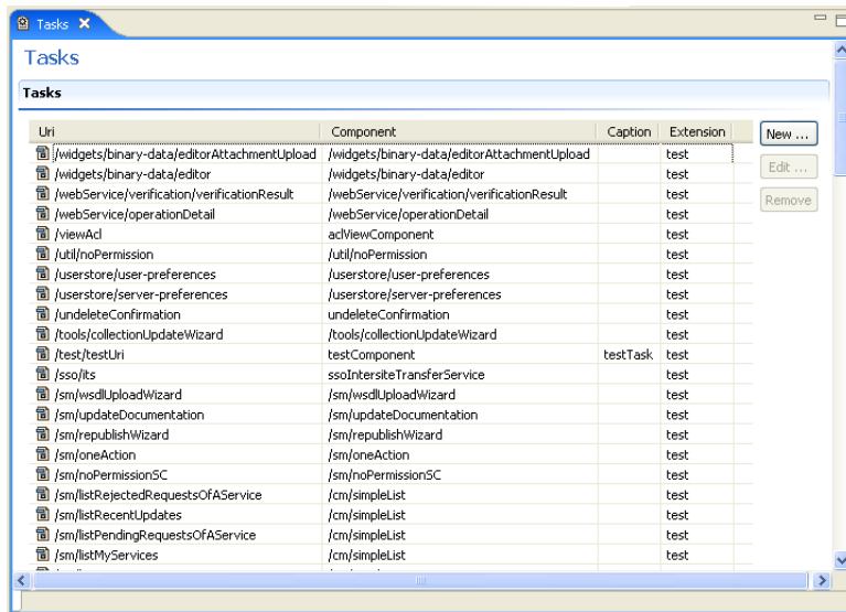
Figure 34. Tasks Editor
