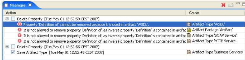
Figure 21. Messages View
