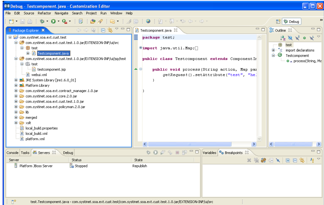
Figure 9. Debug Perspective
