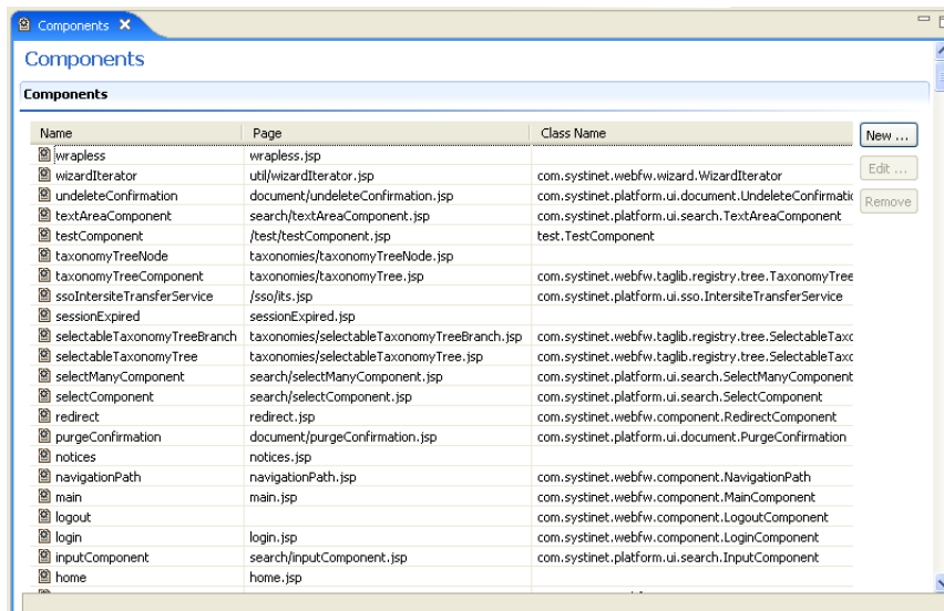
Figure 18. Components Editor
