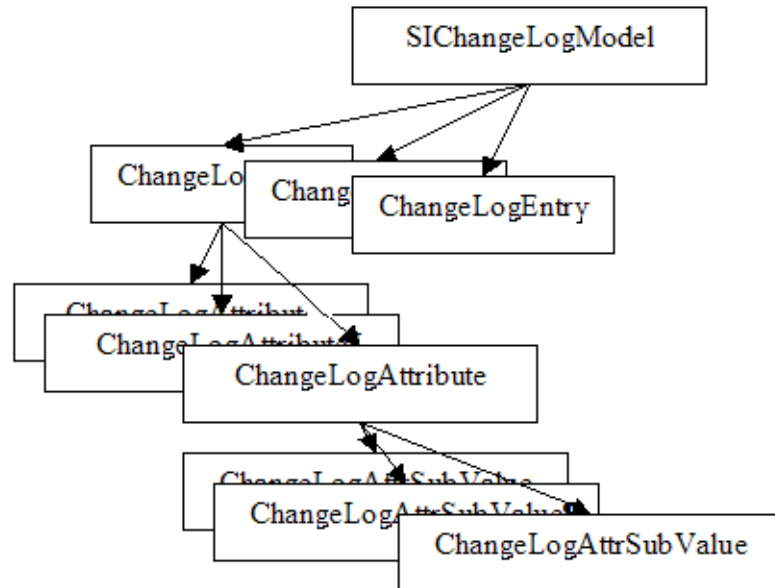
Figure 4 SIChangeLogModel Structure
