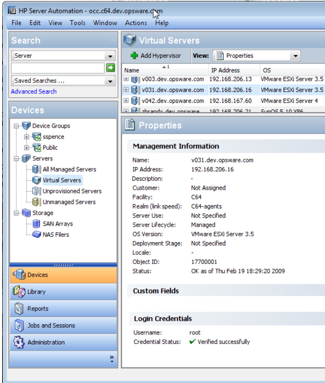
Figure 54 Login Credentials for a VMware ESXi Server
