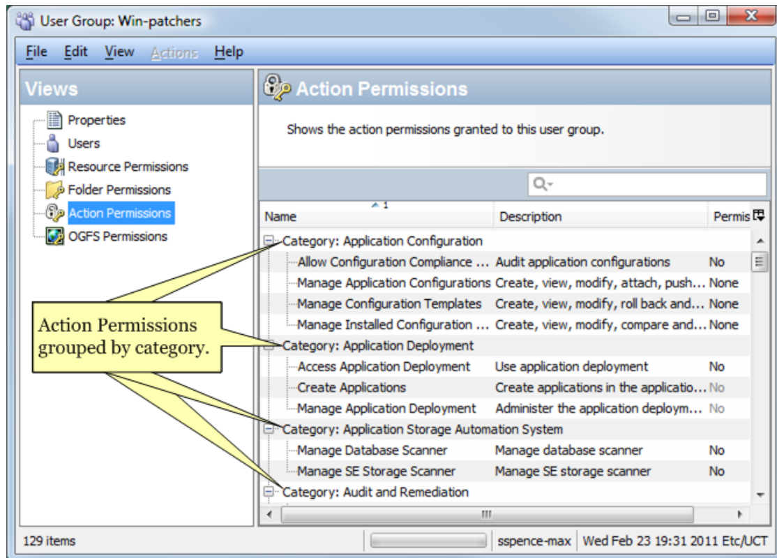
Figure 5. User Group Window - Action Permissions View, Grouped by Category
