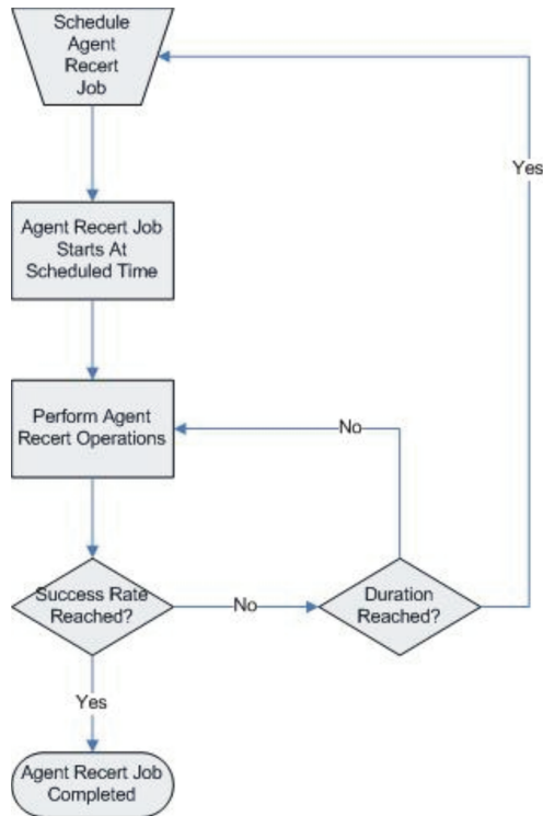
Figure 23. Agent Recertification Job Flow
