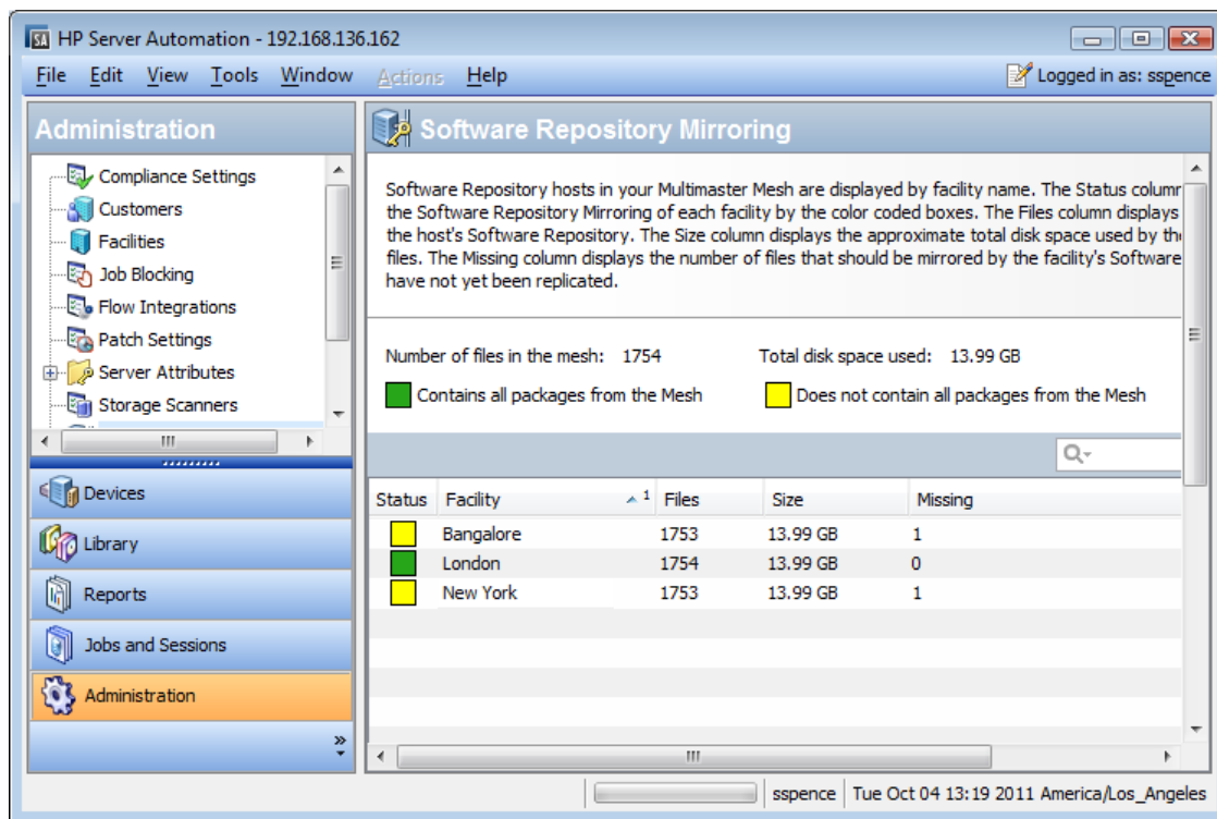
Figure 35. Software Repository Mirroring Status—Out of Sync
