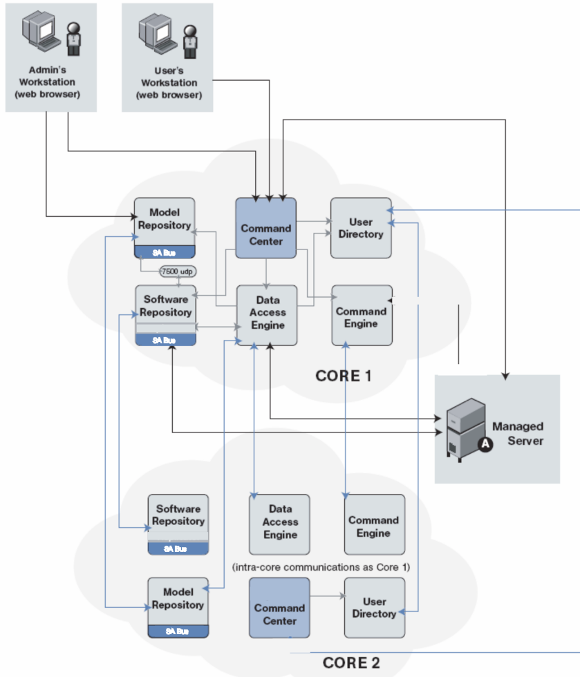
Figure 21. Component Communication
