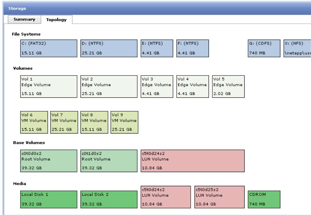
figure 2 Storage Layers
