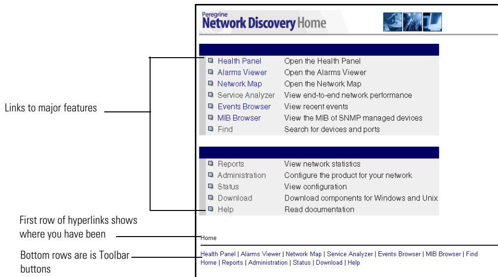
Figure 5-1: Home page
