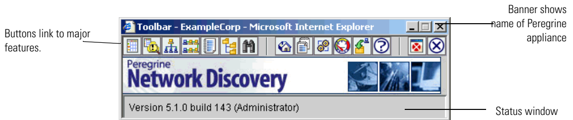
Figure 5-2: Toolbar
