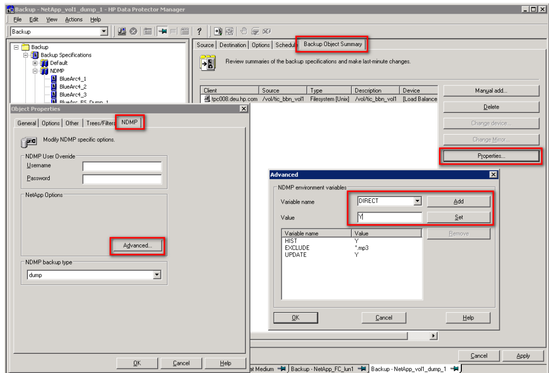
Figure 15: Backup Summary
