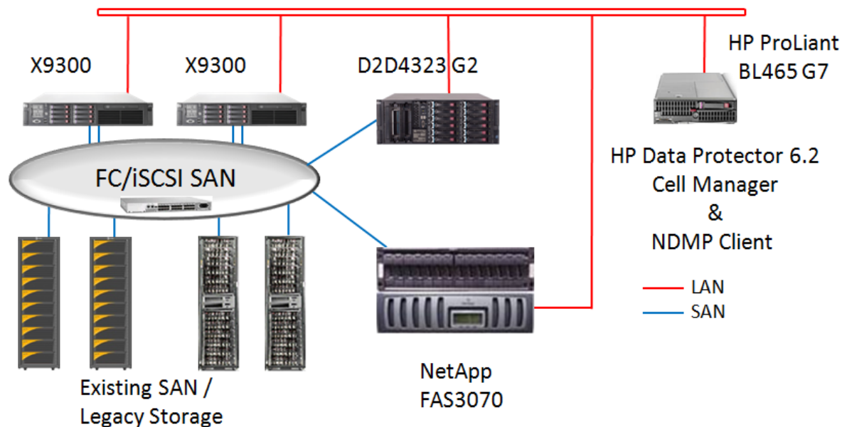
Figure 2: NDMP 2-way backup topology
