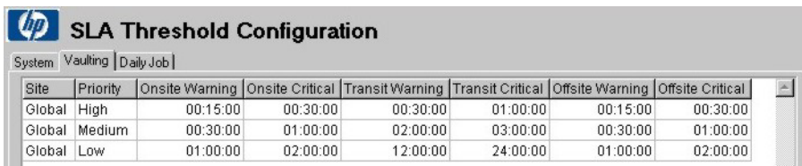
Figure 54 SLA threshold configuration
