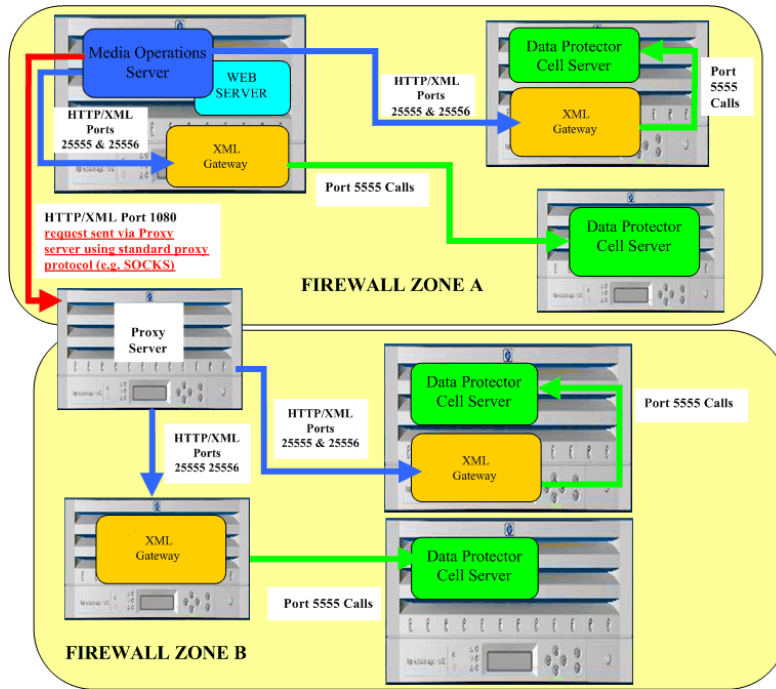
Figure 23 Media Operations deployment options with Data Protector
