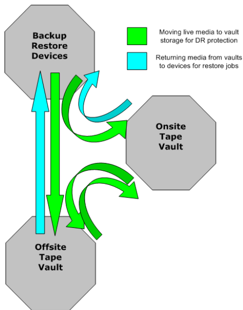
Figure 35 Vaulting jobs media movement
