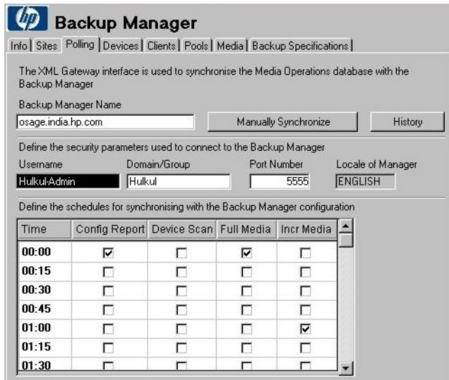
Figure 30 Backup manager - polling
