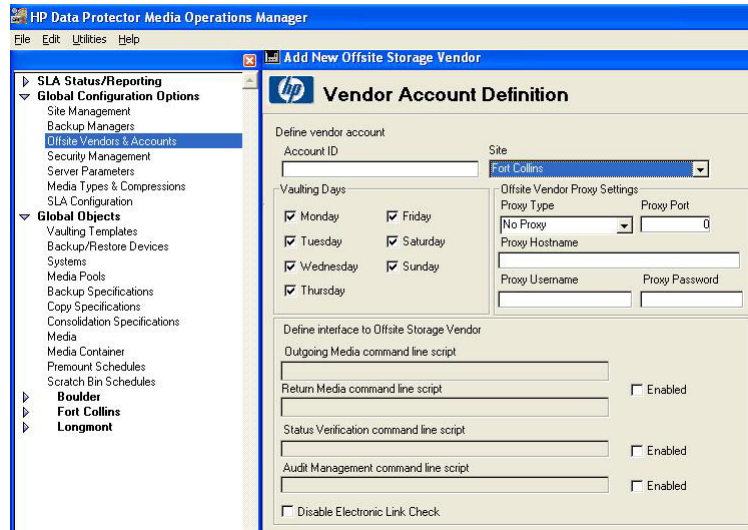
Figure 12 Vendor account definition—generic vendor
