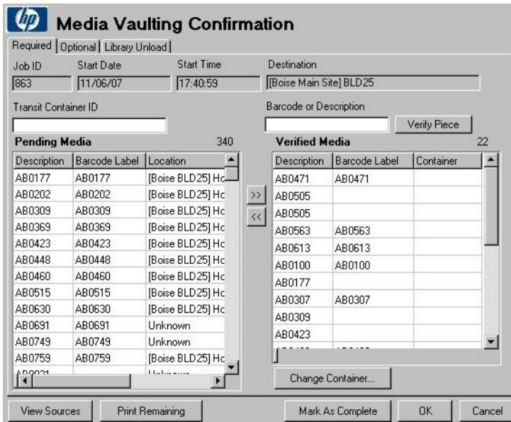
Figure 37 Media vaulting confirmation
