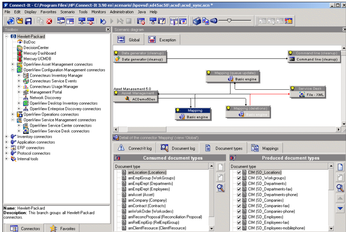
Figure 3.1. Scenario builder - Main window
