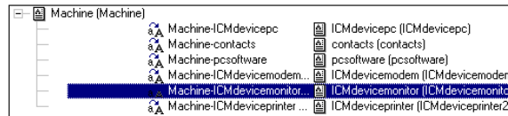
Figure 4.23. Mapping order
