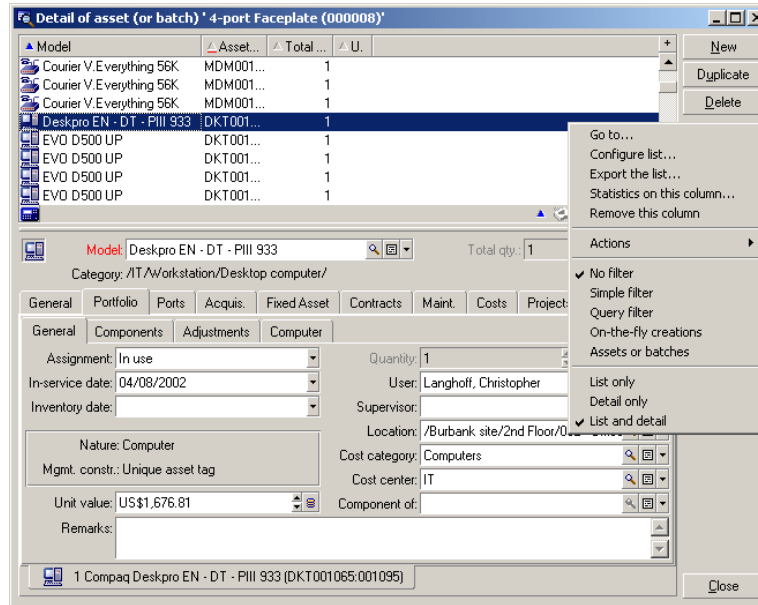
Figure 2.5. Display made up of the list of assets and of a detail
