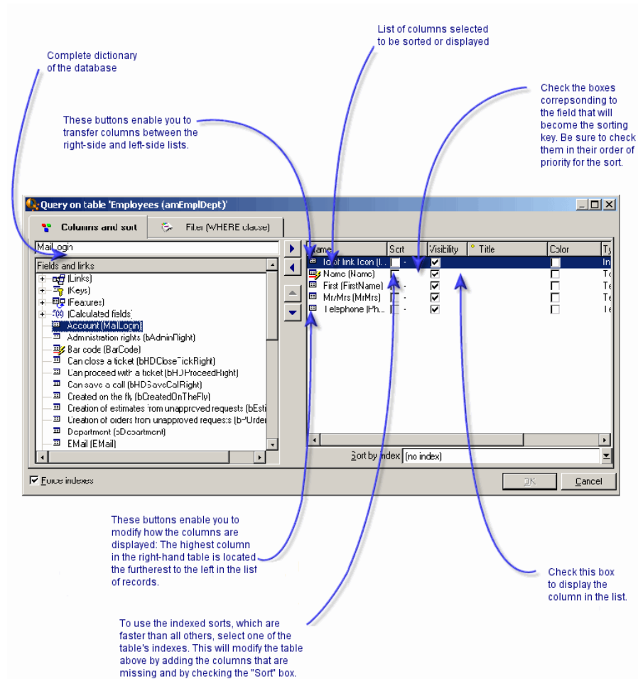
Figure 2.4. Configuring a list
